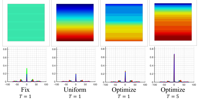
Figure 4: Choice of d_0 s at different locations. The center part indicates the screen under the UDC aperture, and the white edges indicate the normal screen. The display is at 600 DPI. Colors from dark blue to red indicate d_0 s determined by wavelengths from 400 nm to 700 nm.
