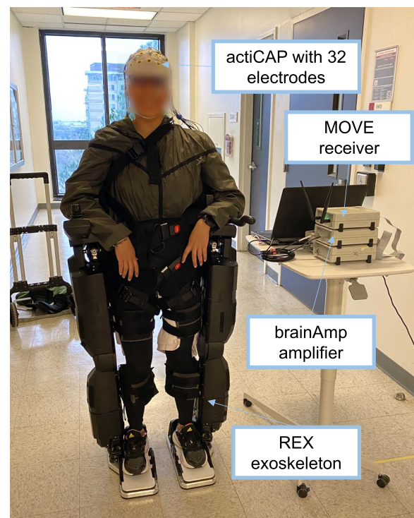
Fig. 1 Equipment employed in the experiments
