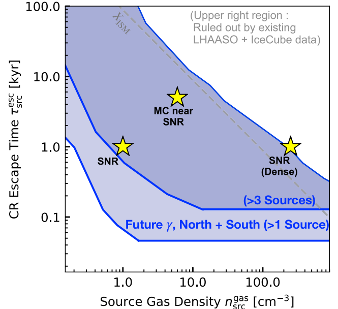
FIG. 8. Sensitivity of SWG0 (or ALPACA) + LHAASO to Galactic hadronic PeVatrons. Same as the left panel of Fig. 6, but we omit constraints from the existing LHAASO and IceCube data for visibility (we instead add a remark in the right top corner). Key takeaway : Future gamma-ray observations are promising to find more than one PeVatron, even if n_{\text{src}}^{\text{gas}} and/or \tau_{\text{src}}^{\text{esc}} is not large.
