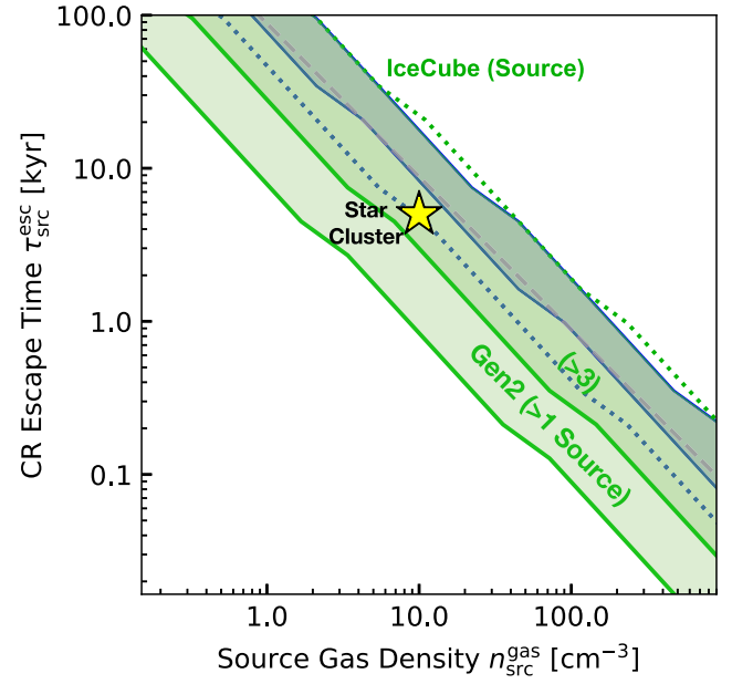
FIG. 14. Same as Fig. 6 (right panel), but for the case of continuous CR injection with \mathcal{N}_{\text{CR}} = 10^2 and R_{\text{src}} = 30 pc.
