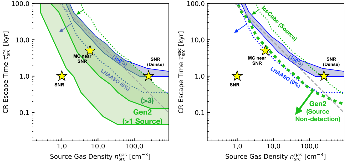
FIG. 6. Sensitivity of Gen2 to Galactic hadronic PeVatrons. Left: the case of detections. Right: the case of nondetections. The other features follow Fig. 3 (left panel). Key takeaways: Over a wide parameter space, it is promising that Gen2 will find more than one PeVatron, though it may find zero. Nondetection by Gen2 would rule out models where 100% of the LHAASO sources are hadronic and also where X_{\text{src}} > X_{\text{ISM}} , but would still allow a wide range of hadronic models.
