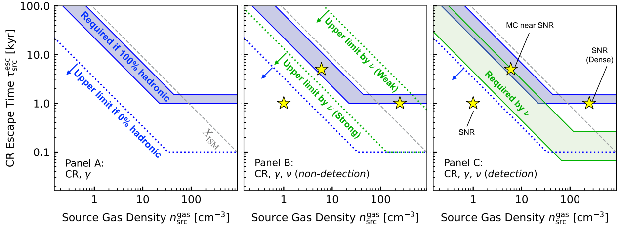
FIG. 2. Schematic constraints in the n - \tau plane for PeV sources. Panel A considers hypothetical gamma-ray source data in light of real CR data. If all gamma-ray sources are hadronic, then the sources must lie within the blue band; if none are, then the sources must lie below the blue dotted line. Regardless of the interpretation of the nature of the gamma-ray sources, the upper right of the plane is excluded. Panels B and C compare hypothetical neutrino source data (green bands/lines, with similar interpretations). The dashed gray line indicates where the column density encountered by CRs in the source ( n_{\text{src}}^{\text{gas}} c \tau_{\text{src}}^{\text{esc}} ) equals that encountered in the ISM before escape from the Milky Way ( X_{\text{ISM}} ), a relevant scale for comparison. Stars indicate possible source classes. For this figure, we assume a CR source rate of 0.03 \text{ yr}^{-1} . This new, semi-model-independent plane allows consistent comparisons of CR, gamma-ray, and neutrino data. See text for details.
