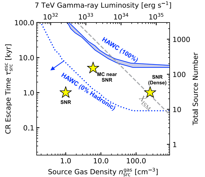
FIG. 5. Constraints from HAWC source measurements (at E_\gamma = 7 TeV). X_{\text{ISM}} is scaled to the value for E_p = 70 TeV. Key takeaway : Large values of n_{\text{src}}^{\text{gas}} and \tau_{\text{src}}^{\text{esc}} are needed to have all HAWC sources to be hadronic, suggesting that leptonic sources may be dominant.
