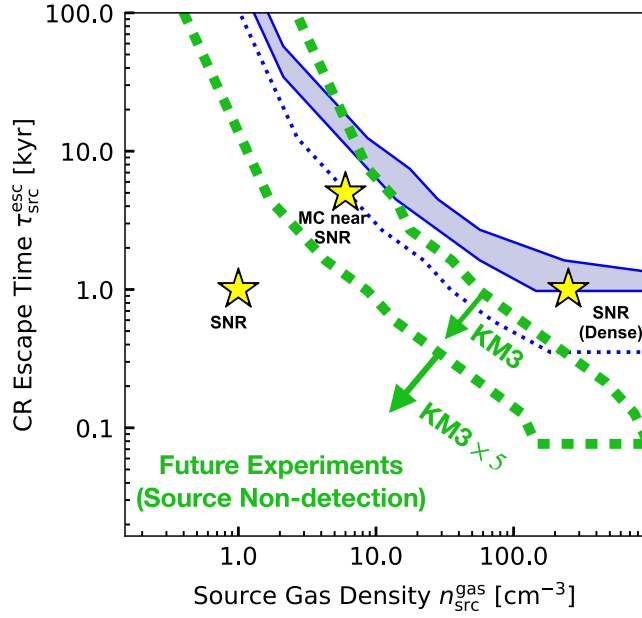
FIG. 7. Projected constraints from future neutrino experiments for the case of nondetection. Labels are same as the right panel of Fig. 6 (except for Gen2) and omitted. Some arrows are removed to improve visibility. The neutrino sensitivities are assumed to be uniform across the sky with values as expected for KM3NeT (marked with “KM3”) and five times better than that (“KM3 \times 5”). Key takeaway : To definitely probe scenario where hadronic PeVatrons are thin, sensitivity better than that of even Gen2 and KM3NeT is needed.
