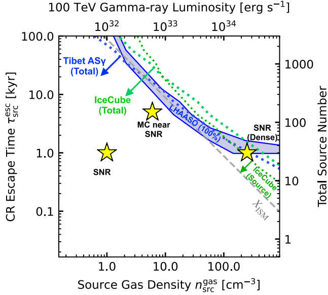
FIG. 4. Same as Fig. 3 (left panel), adding constraints on sources from the Tibet AS \gamma (a measurement) and IceCube (a limit) observations of the Milky Way plane. The alternate axes also apply to the other main text figures. Key takeaway : Constraints from the Milky Way plane emission are important.
