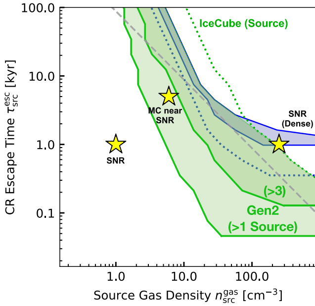
FIG. 13. Same as Fig. 6 (right panel), but for R_{\text{src}} = 30 pc.
