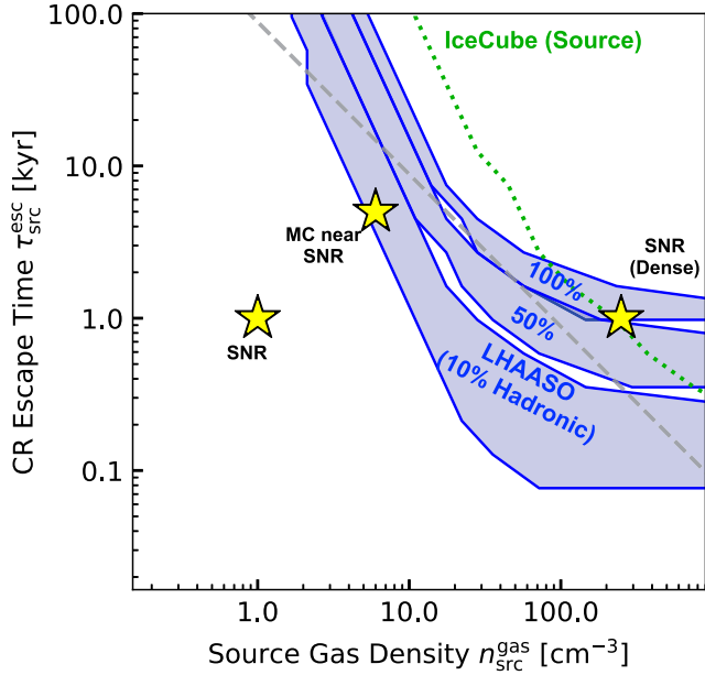
FIG. 10. Same as Fig. 3 (right panel), but for R_{\text{src}} = 30 \text{ pc} .
