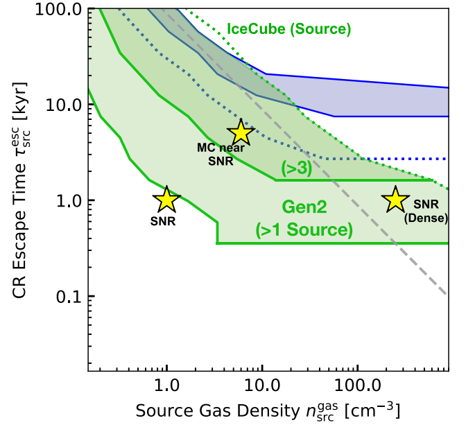
FIG. 12. Same as Fig. 6 (right panel), but for \Gamma_{\text{CR}} = 0.003 \text{ yr}^{-1} .
