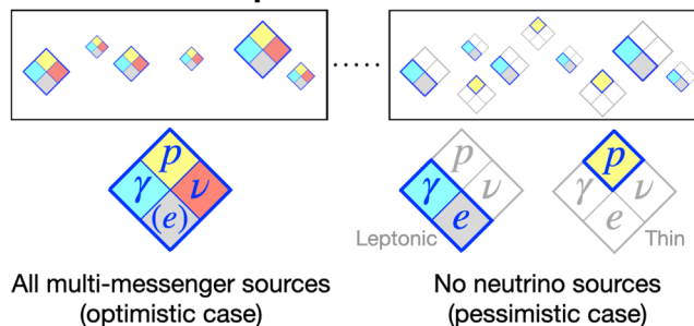
FIG. 1. Possible scenarios for PeV sources. Each diamond is a source, emitting the noted particles. Bottom left shows the “optimistic” case, where all gamma-ray sources are hadronic PeVatrons with neutrino emission. Bottom right shows the “pessimistic” case, where all gamma-ray sources are leptonic and no hadronic PeVatrons produce detectable gamma-ray or neutrino fluxes.
