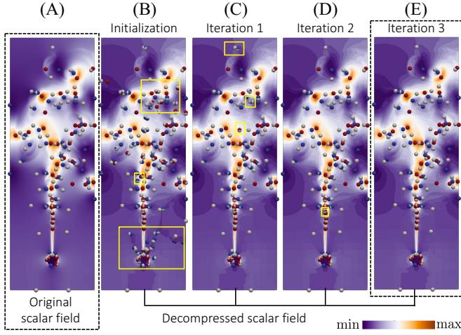
Fig. 12: The compression process of the Heated Flow dataset, with a persistence threshold \varepsilon = 0.02 and a global error bound \xi = 0.05 . (A)-(E): the original scalar field, the decompressed scalar fields in the initialization step, 1st iteration, 2nd iteration, and 3rd iteration, respectively. Local maxima are in red, local minima are in blue, and saddles are in white. Yellow boxes contain false cases.
