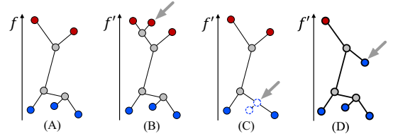
Fig. 1: Examples of false cases (pointed by arrows) in preserving the contour trees during compression. (A) The contour tree that arises from the original scalar field f . (B-D) Contour trees that arise from the decompressed scalar field f' : (B) false positive, (C) false negative, and (D) false type.
