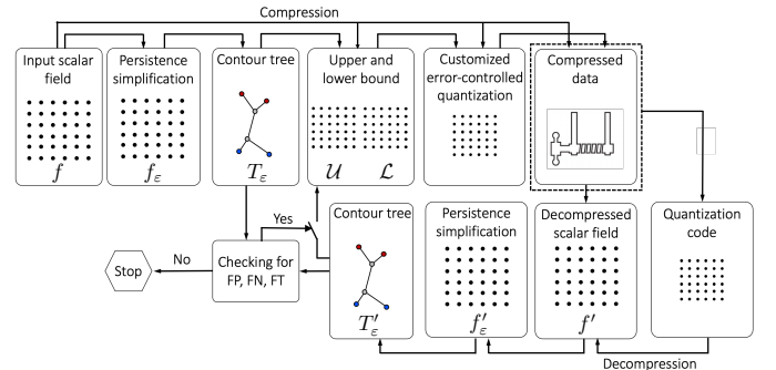
Fig. 5: TopoSZ pipeline for topology-preserving compression.
