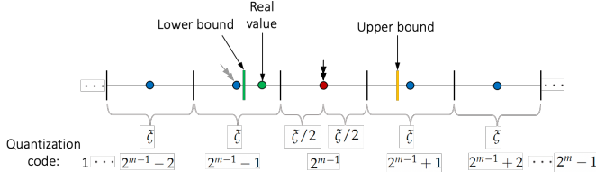
Fig. 8: A customized error-controlled quantization encoder for TopoSZ based on the upper and lower bounds.
