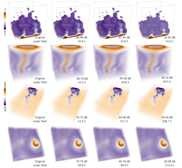
Fig. 9: 3D visualization for the Viscous Fingers (1st row), Tornado (2nd row), Tangaroa (3rd row), and Isabel (4th row) datasets. Columns 1-4: the original data, the decompressed data with high, medium, and low quality, respectively. We also report the PSNR and the compression ratio for each decompressed dataset.
