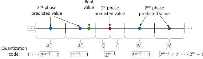
Fig. 2: The design of an error-controlled quantization encoder in the SZ-1.4 based on a linear scaling of the error bounds. Image reproduced from [58, Fig. 2].
