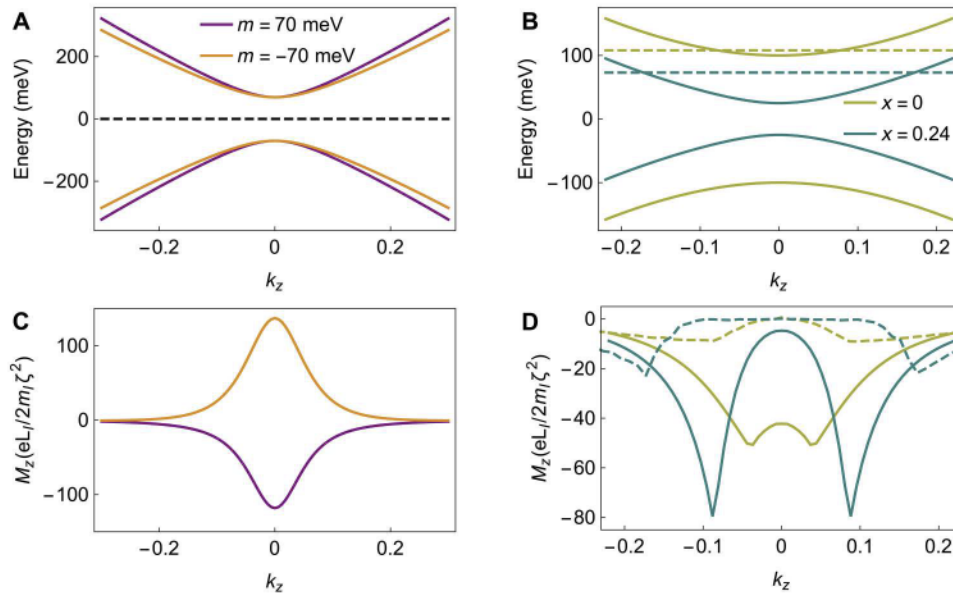
Fig. 4. Phonon magnetic moment from electronic band topology. (A) A generic electronic band structure for a k \cdot p Hamiltonian describing the low energy bulk band structure in \text{Pb}_{1-x}\text{Sn}_x\text{Te} for opposite mass terms with the Fermi level shown by a dashed line. (B) The band structure for the particular case of x = 0 and x = 0.24 where v_F = 1 \text{ eV} , v_3 = 0.3 \text{ eV} , and the Fermi level shown by the dashed line is calculated on the basis of carrier population. (C) Phonon magnetic moment calculated for the Fermi level in the gap for opposite mass terms. The phonon magnetic moment changes sign with the mass term. (D) The topological (solid) and nontopological (dashed) contribution to phonon magnetic moment for the two Sn concentrations in (B). The phonon magnetic moment from the two bands are equal and opposite, and thus, its value is suppressed when Fermi level lies below or above the gap.
