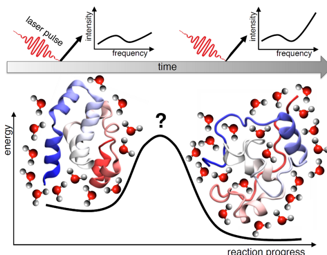
Figure 7. Plot of the free energy G during a reaction (here: protein unfolding). During the reaction, not only the protein structure but also protein hydration is changed, which is probed by THz spectroscopy as a function of time during protein folding.
