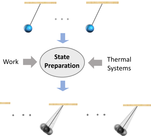
FIG. 1. Preparing a quantum system in a general state requires consumption of both work and coherence. Here, we study the coherence cost of preparing state, when there are no limitations on work consumption. Equivalently, we characterize the minimum rate of consumption of quantum clocks that is needed to prepare a general state, when one does not have access to the standard reference clock.
