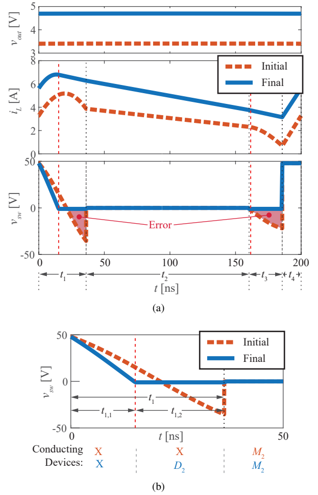
Fig. 4. Example steady-state waveforms of synchronous buck converter (a) before and after state-dependent switching correction and (b) zoomed-in waveforms of initial dead time
