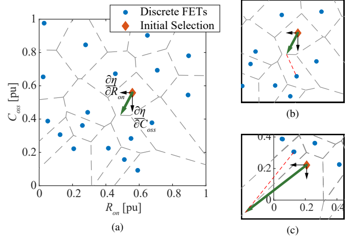
Fig. 6. Example iterative transistor selection from discrete devices. Individual FETs are shown with a voronoi diagram (dashed gray lines) showing the regions closest to each discrete device. Cases of selecting subsequent iteration are shown in (b) and (c)
