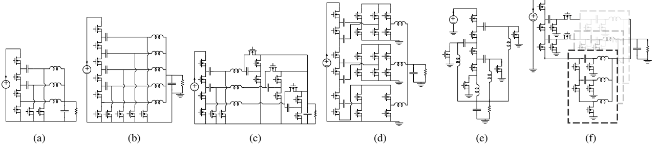
Fig. 10. Topologies included in example 48-to-1 V optimization. 3-phase (a) and 5-phase (b) series capacitor buck [12], series capacitor buck with switched-capacitor step-down [13] (c) LEGO-POL [14] (d) Multi-Inductor Hybrid [15] (e) and Dickson 2 [16]
