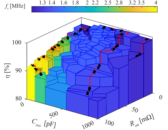
Fig. 9. Paths of iterative convergence to maximum efficiency designs for three starting point for the synchronous buck converter with dead time considered.
