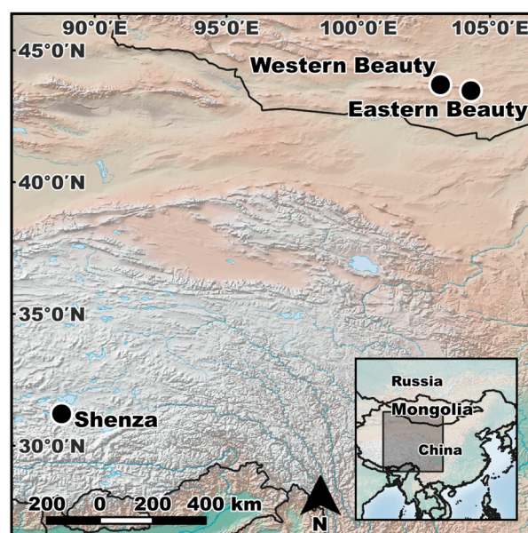
Figure 1. Sampling sites for the Pallas's cat ( Otocolobus manul ) scats included in this study. Scats were collected in Shenza, Tibet Autonomous Region ( n = 1 ) and the Western and Eastern Beauties of Mongolia ( n = 2 and n = 3 , respectively) during noninvasive genetic surveys.
