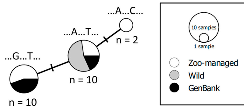
Figure 2. Minimum spanning network of Pallas's cats ( Ootocolobus manul ) at the mitochondrial 12S ribosomal RNA (MT-RNR1; 91 bp) locus. Sequences originated from six wild and ten zoo-managed cats sequenced in this study and six additional sequences from NCBI's GenBank ( n = 22 ). The wild Pallas's cat scats were collected in Shenza, Tibet Autonomous Region ( n = 1 ) and the Western and Eastern Beauties of Mongolia ( n = 2 and n = 3 , respectively). The white, gray, and black coloration of the haplotypes correspond to zoo-managed, wild, and GenBank individuals, respectively. Shared haplotypes are split proportionally based on the number of sequences collected from wild specimens, zoo-managed specimens, or sequences available through GenBank. Each solid branch represents one mutational step between haplotypes. For each haplotype, the nucleotide present at each segregating site is listed above.
