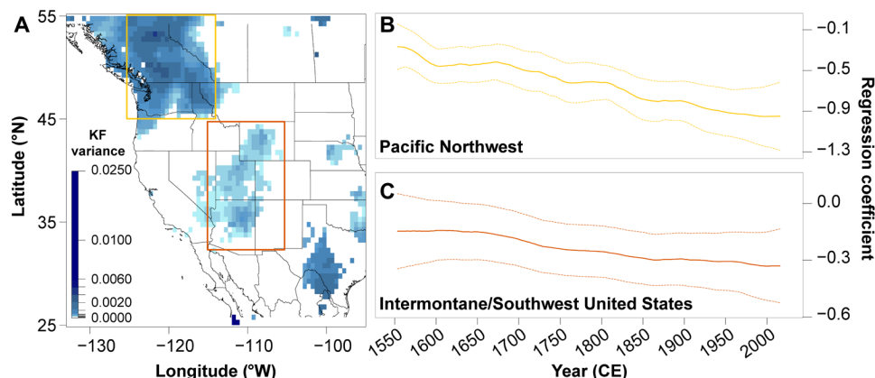
Fig. 3. Dynamic regression modeling using a KF reveals a strengthening relationship between reconstructed maximum temperature and Palmer's modified Drought Severity Index across WNA over the period 1553 to 2020 CE. (A) KF variance resulting from dynamic regression modeling using a KF filter between the LBDA and WNATA time series for each shared grid point. Only variances >0 that also meet the Akaike information criteria are shown in blue. The two selected regions of high variance are denoted with colored boxes. For each of the two identified regions, the regional average of the KF traces (regression coefficients; solid, colored lines) are plotted in (B) for the Pacific Northwest and (C) for the Intermontane/Southwest United States with 95% confidence intervals (dashed, colored lines), where a 30-year high-pass filter was applied to the LBDA and WNATA before regression modeling.
