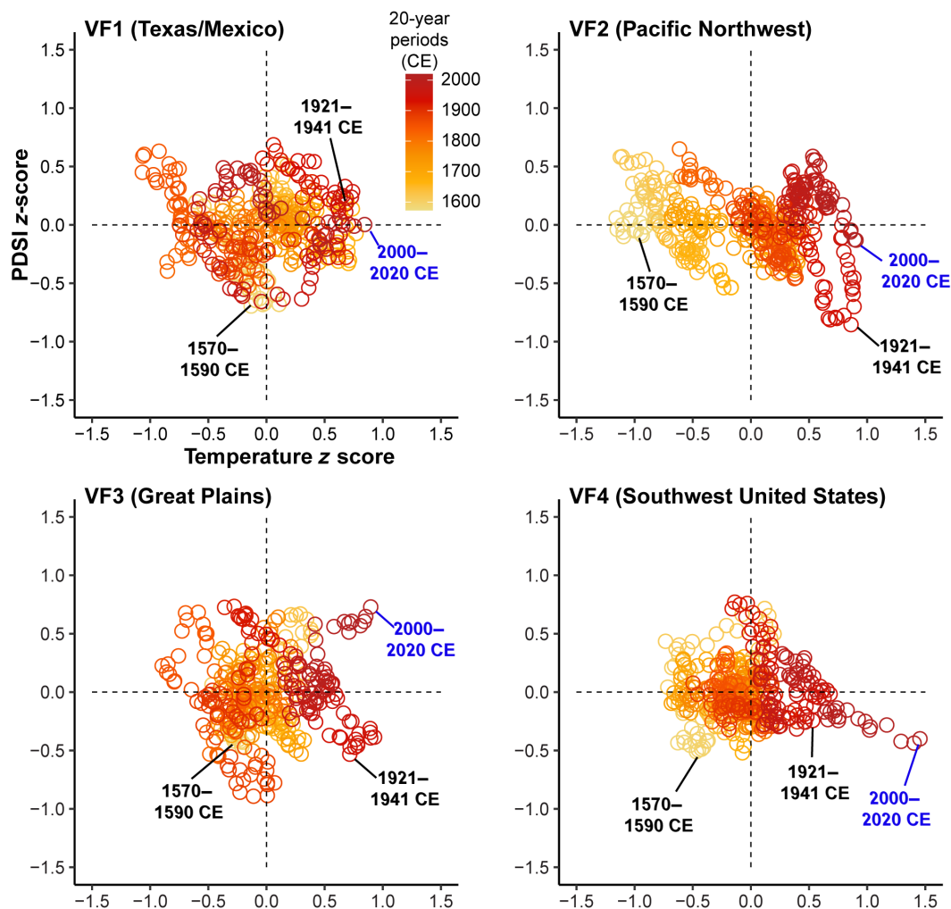
Fig. 2. Bivariate distribution of 20-year moving averages of summer maximum temperature and PDSI across four subregions of WNA. Twenty-year moving averages of regionalized summer temperature z scores from the WNATA and PDSI values from the LBDA are relative to the full period (1553 to 2020 CE). Averages are calculated using a 20-year backward moving window beginning in 2020 CE. For each subregion, the average T_{\max} and PDSI anomaly for the 2000 to 2020 CE period is annotated in blue. Select 20-year periods capturing the Dust Bowl (e.g., 1921 to 1941 CE) and 16th-century megadroughts (e.g., 1570 to 1590 CE) are annotated in black.
