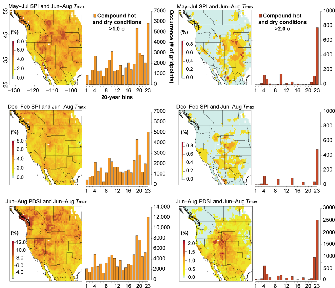
Fig. 4. Historical occurrence of compound hot drought (hot and dry conditions) across WNA since 1553 CE. The fractional probability of occurrence of compound hot and dry conditions is mapped, where in any given year over the period 1553 to 2016 CE, each grid point location experiences concurrent warm season (May to July; top row ), cool season (December to February; middle row ), standardized precipitation index deficits, or warm season (JJA; bottom row ) PDSI deficits and positive summer maximum temperature anomalies exceeding 1.0\sigma ( left column ) and 2.0\sigma ( right column ). Counts of occurrence at the grid point level of compound warm and dry summer conditions are plotted in 20-year bins to the right of each map. For bar plots, year corresponding to bin numbers 1 to 23 are: 1) 1557 to 1576, 2) 1577 to 1596, 3) 1597 to 1616, 4) 1617 to 1636, 5) 1637 to 1656, 6) 1657 to 1676, 7) 1677 to 1696, 8) 1697 to 1716, 9) 1717 to 1736, 10) 1737 to 1756, 11) 1757 to 1776, 12) 1777 to 1796, 13) 1797 to 1816, 14) 1817 to 1836, 15) 1837 to 1856, 16) 1857 to 1876, 17) 1877 to 1896, 18) 1897 to 1916, 19) 1917 to 1936, 20) 1937 to 1956, 21) 1957 to 1976, 22) 1977 to 1996 and 23) 1997 to 2016 CE.
