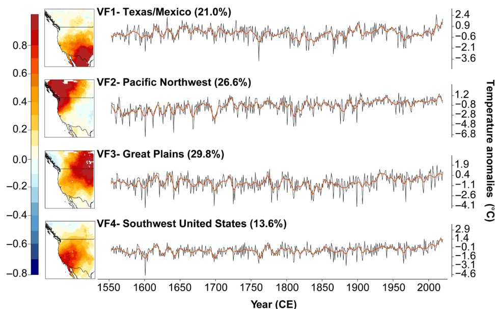
Fig. 1. Subregional expression of reconstructed temperatures across WNA since 1553 CE. (Left) First four varimax-rotated EOF factor scores (ranging from -1.0 to +1.0 ) are mapped and labeled with the variance explained by each factor. (Right) Annual (thin black line) and 10-year low pass-filtered (thick red lines) reconstruction time series of JJA maximum temperatures for four major regions of WNA, spanning the period 1553 to 2020 CE. Anomalies are relative to the 1951 to 1980 CE mean. The four regional time series are calculated using the rotated varimax factor loadings over the period 1901 to 2000 CE.
