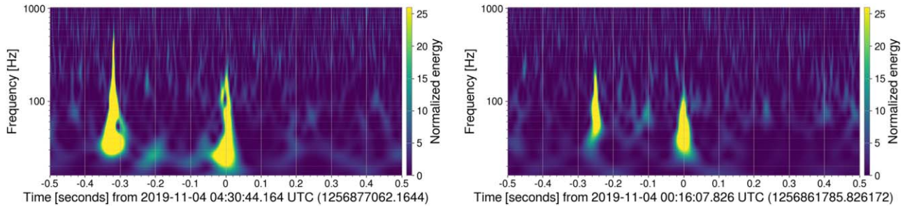
Figure 2. Spectrograms of the LHO data (left) at the time of the most significant cluster found in the on-source window of burst 2653, and an instrumental artifact appearing also in the LHO data (right). The time separation between these two events is \sim 15,277 s, which is larger than the size of the background window in our analysis, and therefore the instrumental artifact was not included in the background. These two spectrograms display very similar structure, with similar double short-duration transients separated in both cases by \sim 0.3 s. Several instrumental artifacts of this nature are found by Omicron (Robinet et al. 2020) within the day of burst 2653. The second most significant cluster in the same delayed on-source analysis of burst 2653 also has this same double-peaked structure.
