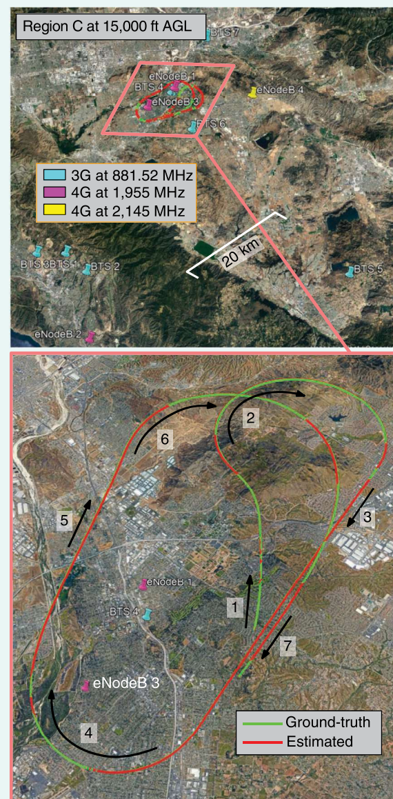
FIG 10 Experimental layout and results in Region C showing BTS and eNodeB positions, true aircraft trajectory, and aircraft trajectory estimated exclusively using cellular SOPs. The aircraft traversed a total distance of 55 km in 8.5 min during the experiment. The position RMSE over the entire trajectory was found to be 15.44 m.
