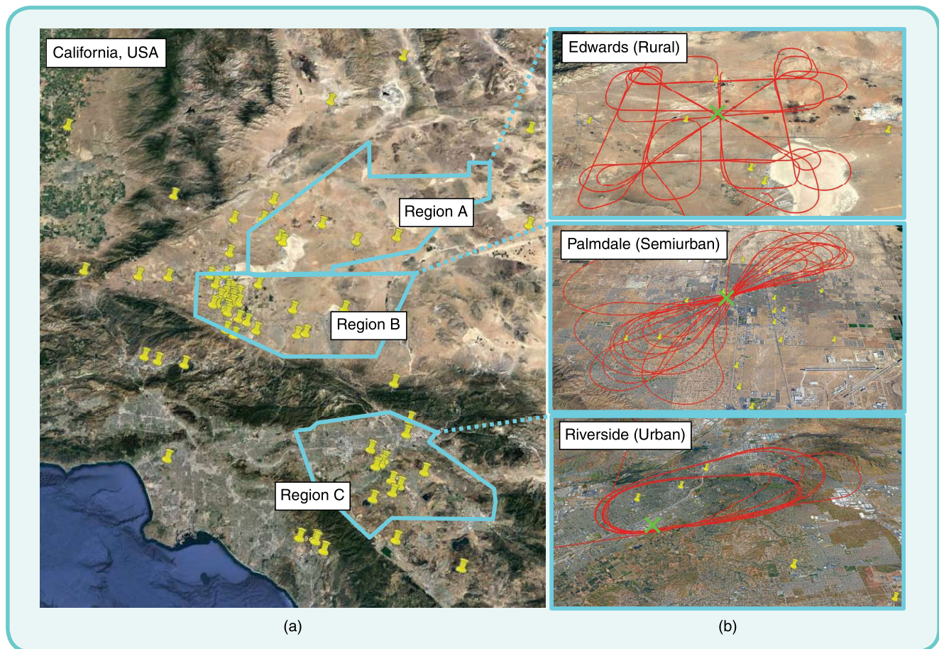
FIG 2 (a) Regions A, B, and C in which the flight campaigns took place. The yellow pins represent 3G and 4G cellular towers that were mapped and analyzed in this study. (b) The aircraft trajectories in all regions (shown in red). Geographic points of interest in each region, shown by green crosses, were chosen according to the designed trajectories.
