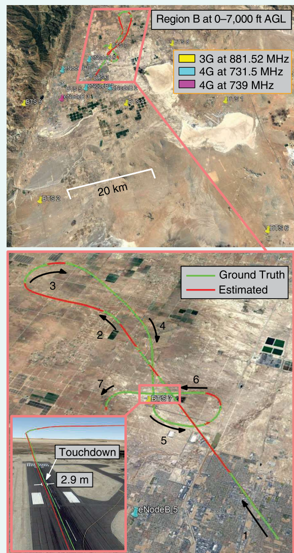
FIG 7 Experimental layout and results in Region B showing BTS and eNodeB positions, true aircraft trajectory, and aircraft trajectory estimated exclusively using cellular SOPs. The aircraft traversed a total distance of 57 km in 11 min during the experiment. The position RMSE over the entire trajectory was found to be 4.96 m. Note that the position estimate on touchdown is less than 3 m away from the true aircraft position and is well within the runway.
