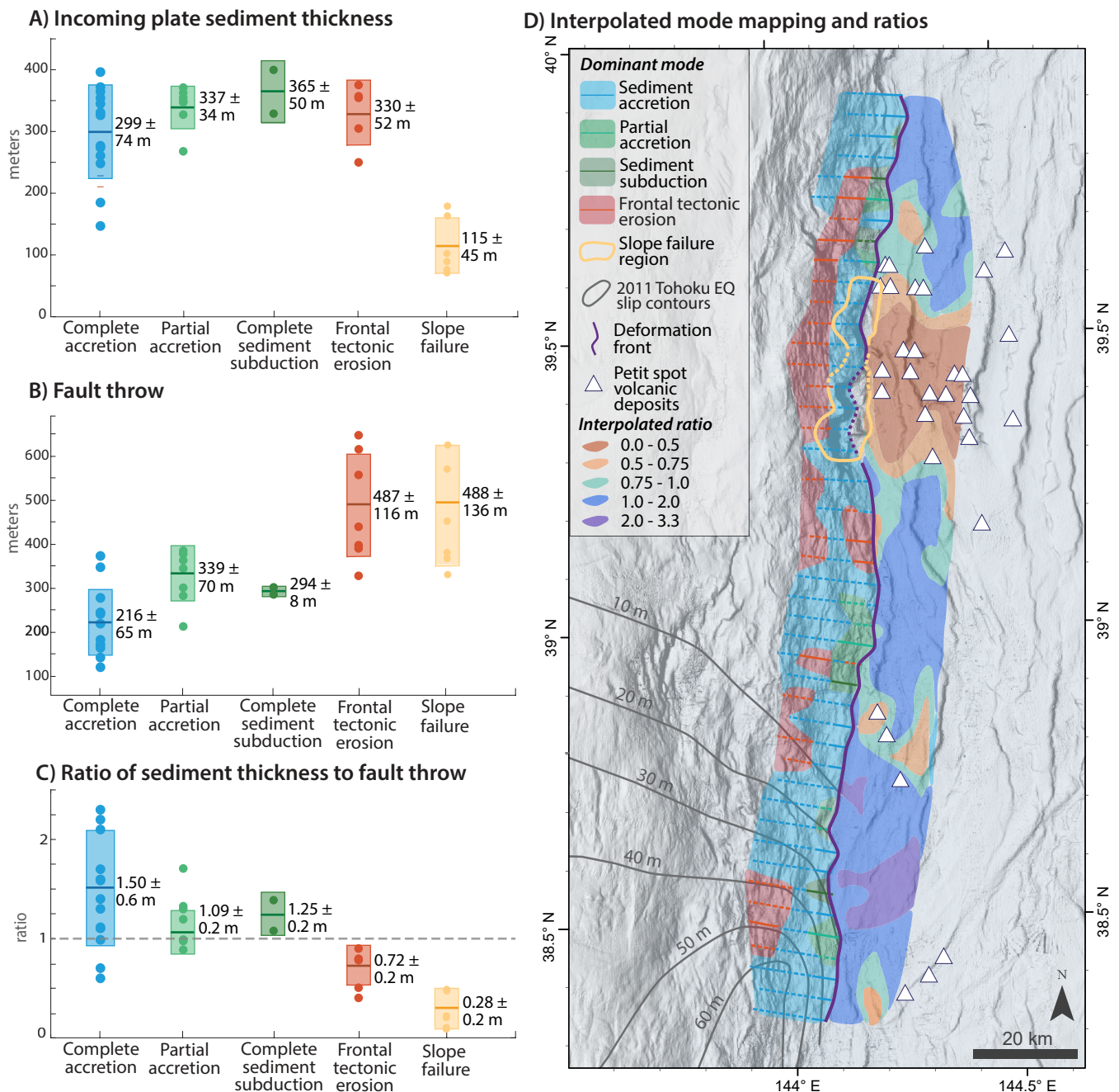
Figure 6 Comparisons between sediment thickness, fault throw, and mode of frontal prism deformation at the trench. Box plots (A - C) include individual measurements (points), weighted averages (horizontal line), and 2\sigma_w uncertainty (boxes). See Figure 4 for measurement locations. A. Sediment thickness as a function deformation mode. Average sediment thickness is the smallest outboard of regions with slope failures. Average sediment thickness is similar in regions experiencing all other modes. B. Fault throw as a function of deformation mode. Portions of the prism experiencing complete accretion have the smallest average fault throw, followed by partial accretion and full sediment subduction, frontal tectonic erosion, and regions with slope failures. C. Ratio of sediment thickness to fault throw as a function of deformation mode. Regions experiencing complete accretion, partial accretion, and complete sediment subduction have ratios >1 . Regions experiencing tectonic erosion or slope failure have ratios <1 . D. Map of dominant prism deformation mode, interpolated sediment thickness to fault throw ratio on the incoming plate (1km grid), and slip contours for the 2011 Tohoku earthquake (after Iinuma et al., 2012).
