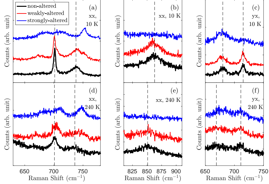
FIG. 6. Raman scattering from phonon modes above 600 \text{ cm}^{-1} in energy. We have not been able to assign an eigenvector to all of these modes, but based on their relatively high energy and the mode assignments in Ref. [12], we believe they must all involve stretching of the in-plane Ir-O bonds. Vertical dashed lines indicate the energies of the phonons in the non-altered sample.
