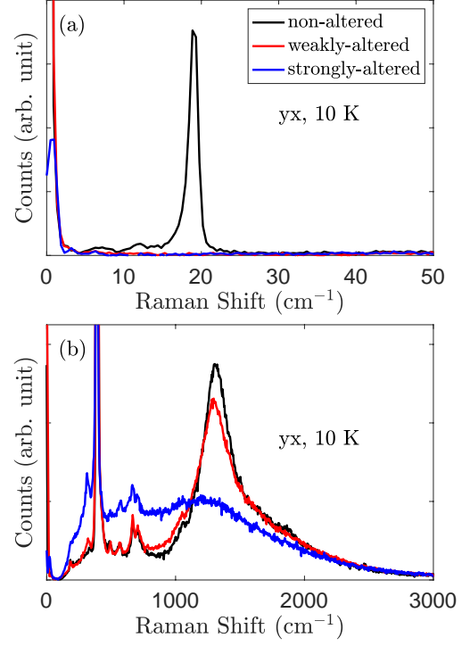
FIG. 4. One-magnon (a) and two-magnon (b) Raman scattering at 10 K. One-magnon scattering appears to be absent in the field altered samples, at least down to our energy cutoff of \sim 5 \text{ cm}^{-1} .
