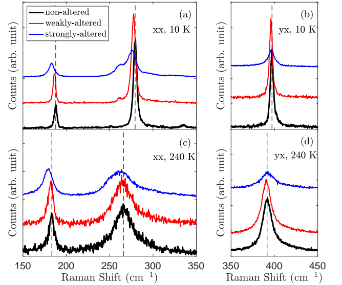
FIG. 5. Raman scattering from phonons which bend the in-plane Ir-O bonds in the polarization geometries xx ((a) and (c)) and yx ((b) and (d)). Vertical dashed lines indicate the energies of the phonons in the non-altered sample.
