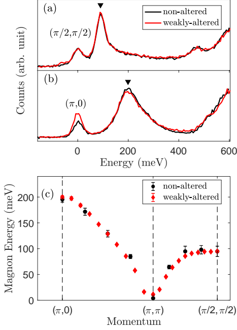
FIG. 3. Raw RIXS data from a non-altered and weakly altered sample at (\pi/2, \pi/2) (a) and (\pi, 0) (b). Black triangles mark the positions of the peaks from one-magnon scattering. At both zone-boundary points, the peak energies match nearly perfectly, suggesting that short-range in-plane couplings are unchanged in the weakly altered sample. The magnon dispersion in (c) shows no major differences between the weakly altered and non-altered samples. Dispersion data on the non-altered sample are adapted from [16].
