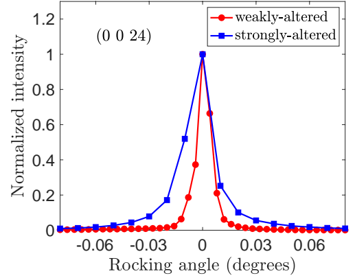
FIG. 8. Rocking scans through the (0 0 24) structural Bragg reflection at 300 K. The widths of these peaks are .007^\circ and .014^\circ for the weakly altered and strongly altered samples, respectively. The difference between the two samples is within systematic uncertainty of the measurement.
