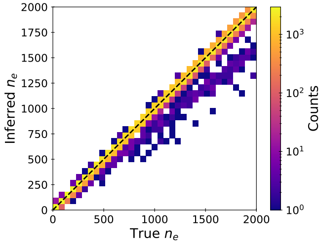
Figure 4: A 2-dimensional histogram showing the results of the inference on the test dataset after the autoencoder has been trained. The dotted line is an exact inference of the number of electrons in the gas gap.
