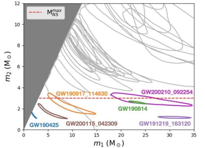
Figure 4. The inferred 90% credible regions of the component masses for all GWs with p_{astro} > 0.5 from O3 are shown in gray (Abbott et al. 2021a, 2021c, 2023). The red dashed line marks the upper bound of m_2 allowed for our classification of systems with a possible neutron star component, which are marked by colored contours.
