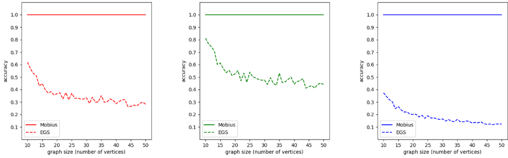
(a) Generalization study for the path benchmark. (b) Generalization study for the connected benchmark. (c) Generalization study for the scc benchmark.
