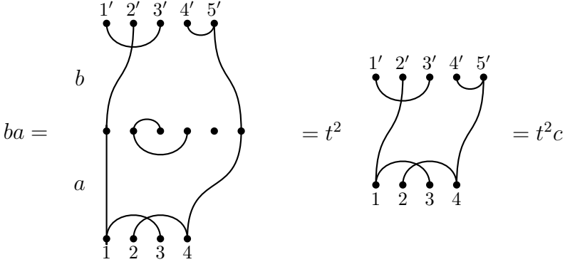
Fig. 7. Composition ba = t^2 c , where the partition c is shown on the right, c = \{\{1, 3, 2'\}, \{2, 4, 4', 5'\}, \{1', 3'\}\} . The coefficient t^2 comes from removing two connected components in the middle of the ba diagram that connect to neither bottom nor top points.
