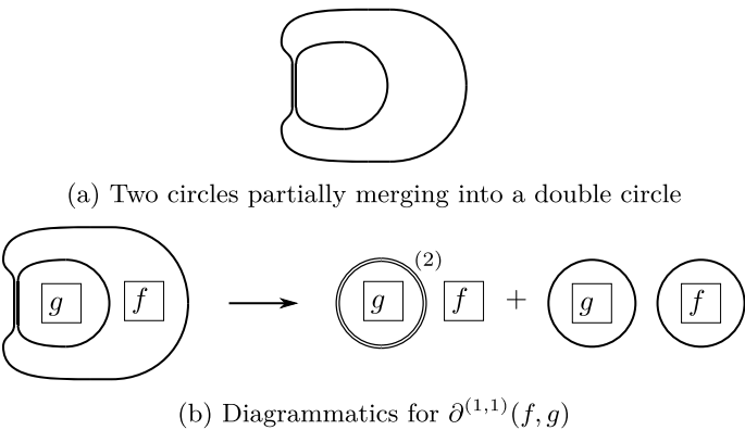
Figure 50: The operator \partial^{(1,1)} , given by formula (74), applied to a pair of functions f, g .
