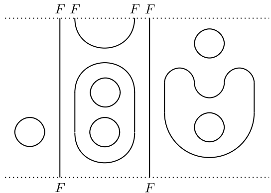
Figure 9: A natural transformation from F^2 to F^4 described by a diagram of 3 arcs and 7 embedded circles. Any such system can be further transformed via isotopies into a form where each circle has a unique maximum and minimum for the projection on the y -axis and each arc has at most one such extremum (none if it connects a top F with a bottom F ).
