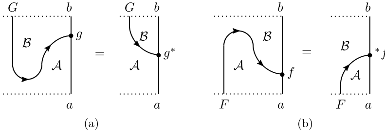
Figure 64: (A) the dual g^* of a morphism g , given by composing with the natural transformation \delta_2: \mathrm{Id}_{\mathcal{A}} \longrightarrow GF , see Figure 2 and Section 2.1; (B) the inverse operation f \mapsto {}^*f .
