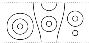
Figure 35: A diagram in \mathbb{U}_2^4 corresponds to an element of \mathbb{B}_2^4 together with circle diagrams in each region.
