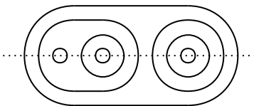
Figure 13: A diagram invariant under the reflection about the (dotted) horizontal axis.
