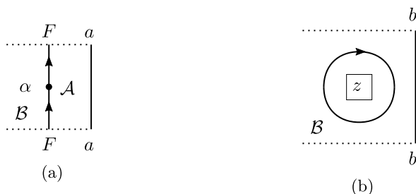
Figure 71: In (A), the four-valent vertex is simplified to parallel lines when the morphism Fa_1 \longrightarrow Fa_2 is \alpha_a: Fa \longrightarrow Fa . In (B), diagrammatics for the morphism \text{tr}_B(z)b: b \longrightarrow b .
