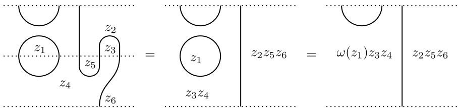
Figure 20: The composition vu of the diagrams from Figure 19 in \mathrm{SU}_\omega .
