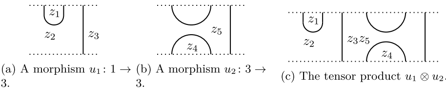
Figure 21: The tensor product of two morphisms in \mathrm{SU}_\omega .
