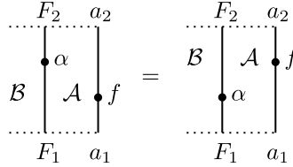
Figure 65: The property of a natural transformation \alpha: F_1 \Longrightarrow F_2 is the isotopy (commutativity) condition that the dots denoting \alpha and f on parallel vertical lines can slide past each other.
