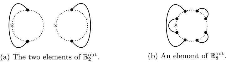
Figure 22: Examples of outer matchings.
