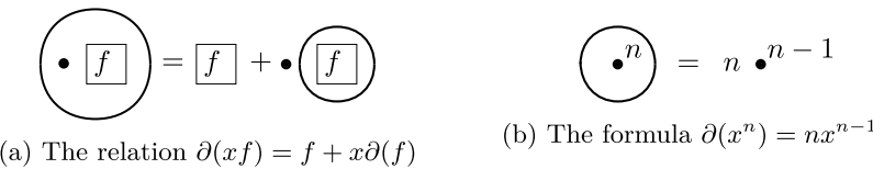
Figure 42: Derivation diagrammatics, multiplication by \bullet = x .
