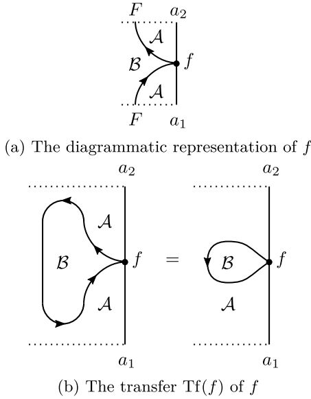
Figure 66: Transfer map diagrammatics for a morphism f: Fa_1 \longrightarrow Fa_2 .
