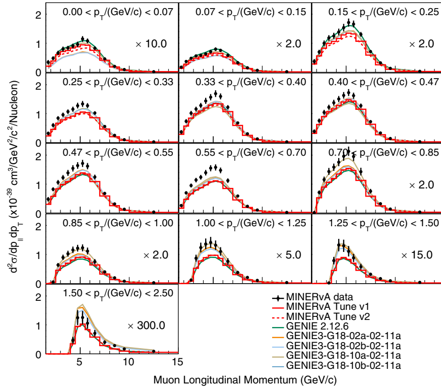
FIG. 7. Double differential cross section as a function of muon longitudinal momentum in bins of muon transverse momentum shown for GENIE 2 and tuned models along with GENIE 3 (v3.0.6) models.
