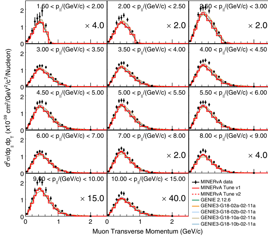
FIG. 4. Double differential cross section as a function of muon transverse momentum in bins of muon longitudinal momentum shown for GENIE 2 and tuned models along with GENIE 3 models.
