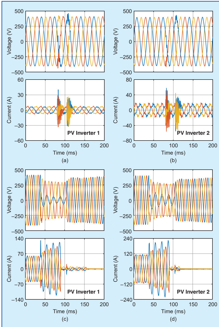
figure 8. Using synchro-waveforms to monitor two distribution-level IBRs. (a) and (b) Simultaneous dynamic waveform response of the two PV units during a system-wide subcycle disturbance. (c) and (d) Simultaneous waveform response of two PV units that cease production when a fault impacting the entire local subtransmission system occurs.
