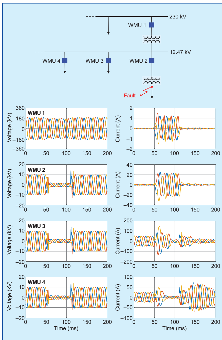
figure 9. Synchro-waveforms for voltage and current that are captured by four WMUs across the 230-kV and 12.47-kV network buses during a fault.
