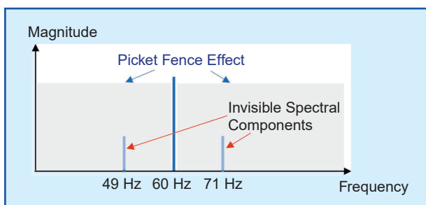
figure 11. Spectral components of voltage oscillation. The components at 49 Hz and 71 Hz can be seen only in synchro-waveforms and not in synchrophasors.
