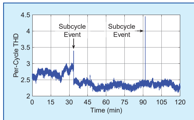
figure 7. The per-cycle THD in a continuous stream of synchro-waveforms. Two subcycle events are marked.
