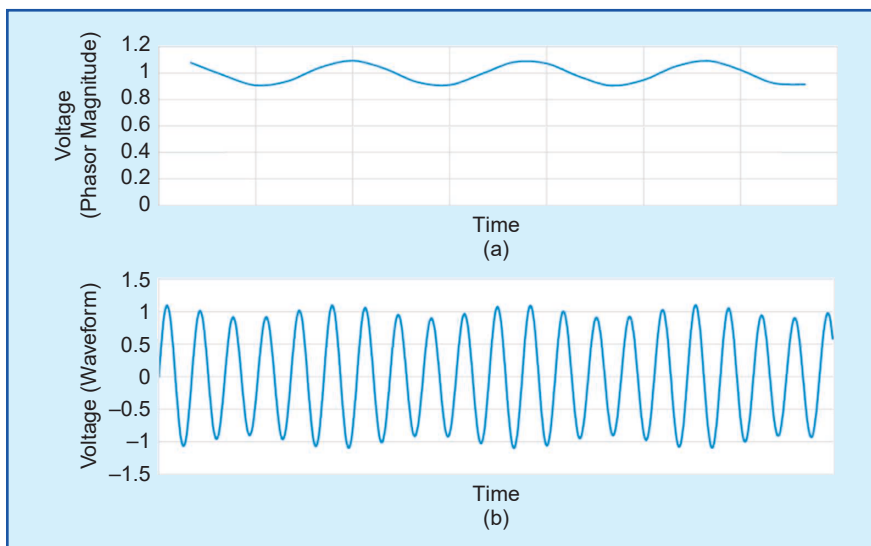
figure 10. Voltage oscillation, as perceived from (a) phasor's perspective and (b) waveform's perspective.
