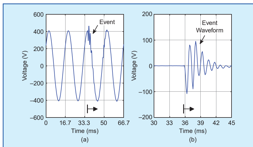
figure 4. (a) Real-world voltage waveform during an event and (b) its extracted event waveform.
