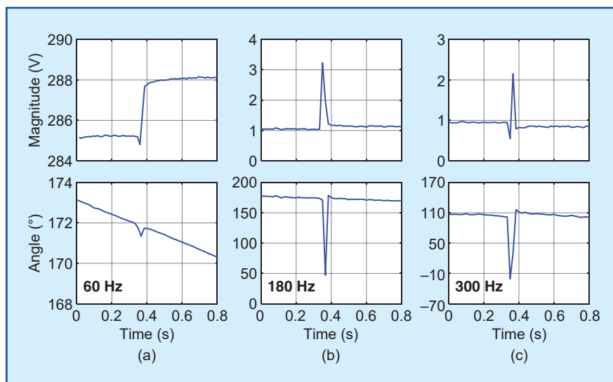
figure 6. Fundamental and harmonic synchrophasor signatures of an event at different frequencies: (a) fundamental frequency, (b) third harmonic, and (c) fifth harmonic.
