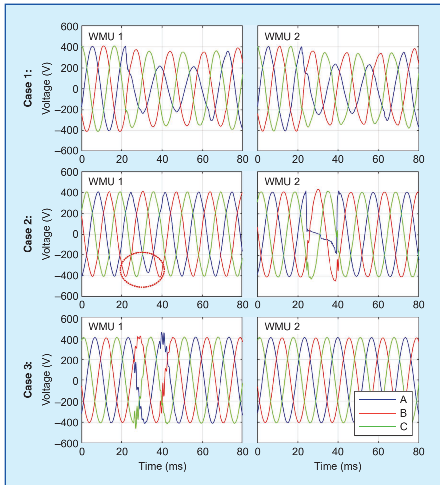
figure 3. Examples of voltage synchro-waveforms from two distribution-level WMUs.
