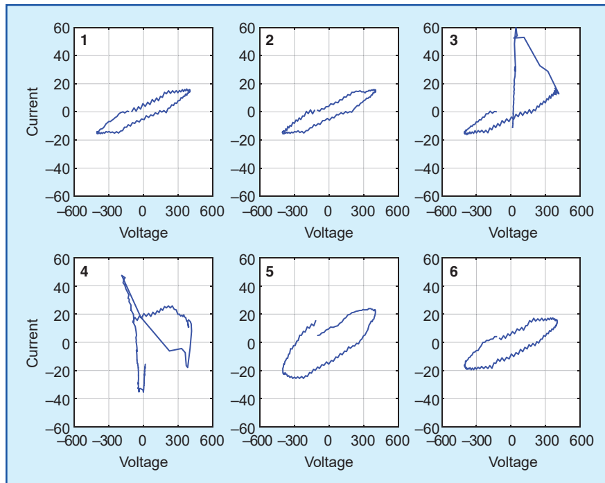
figure 5. Per-cycle Lissajous graphs for voltage waveform (in volt) and current waveform (in amp) during six cycles. A transient event occurs at cycle 3.
