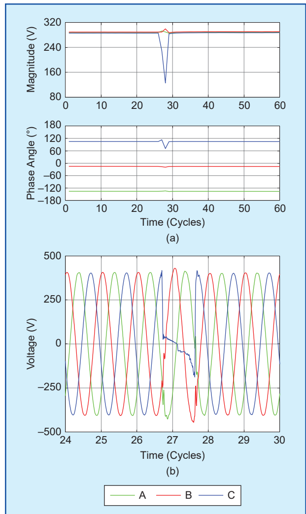
figure 1. Comparing voltage phasors and raw voltage waveforms during a temporary fault: (a) phasor representation in the form of voltage sags and (b) the raw waveforms.
