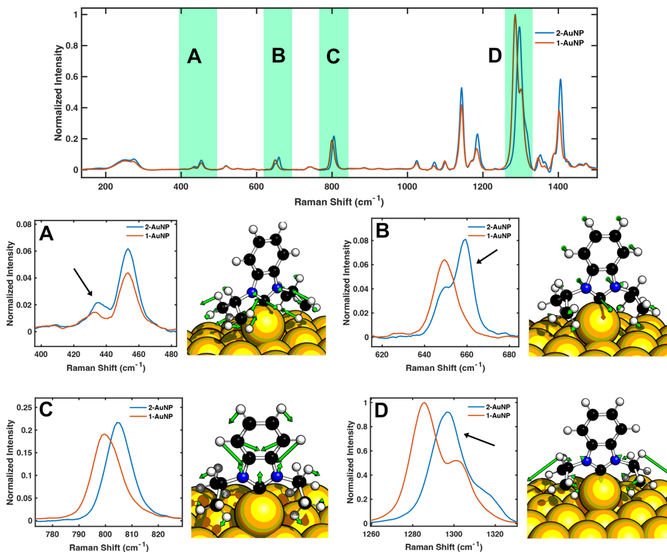
Fig. 2. Comparison of experimentally measured SERS vibrational spectra of ^{13}\text{C} -carbene labelled and natural abundance NHCs on gold nanoparticles, 1-AuNP and 2-AuNP , respectively. Top: Full range of relevant regions with highlighting (green) that show clear isotopic shifts. A. Close-up of 430/433 \text{cm}^{-1} peak and corresponding calculated vibrational mode. B. Close-up of 649/659 \text{cm}^{-1} peak and corresponding calculated vibrational mode. C. Close-up of 799/805 \text{cm}^{-1} peak and corresponding calculated vibrational mode. D. Close-up of 1286/1297 \text{cm}^{-1} peak and corresponding calculated vibrational mode.
