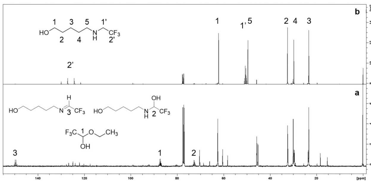
Figure 1. a) Observed equilibrium of trifluoroacetaldehyde ethyl hemiacetal with the imine and hemiaminal intermediates. b) 2° amine after NaBH 4 reduction and separation.
