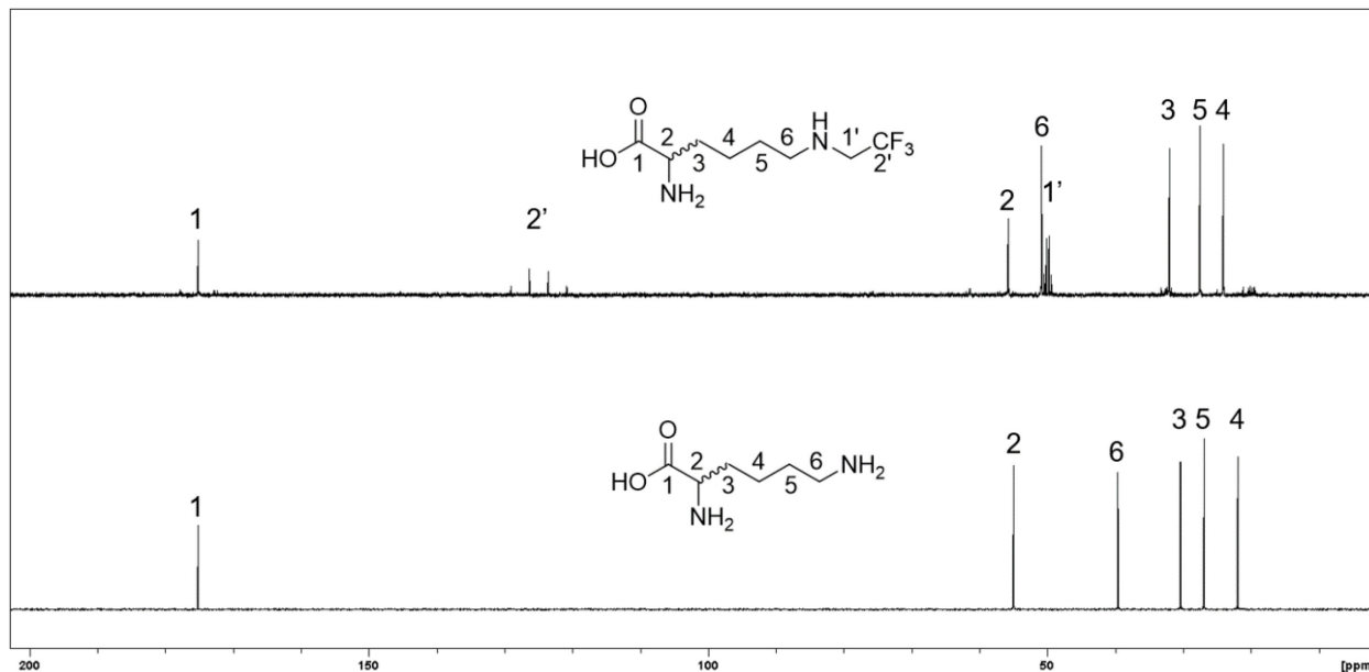
Figure 3. ^{13}\text{C} NMR of D,L -lysine (bottom) and N^\epsilon -(2,2,2-trifluoroethyl)- D,L -lysine ( 7 , n = 2 , top) (pulse prog. zgpg30 , 90% \text{H}_2\text{O} /10% \text{D}_2\text{O} , 400 MHz).
