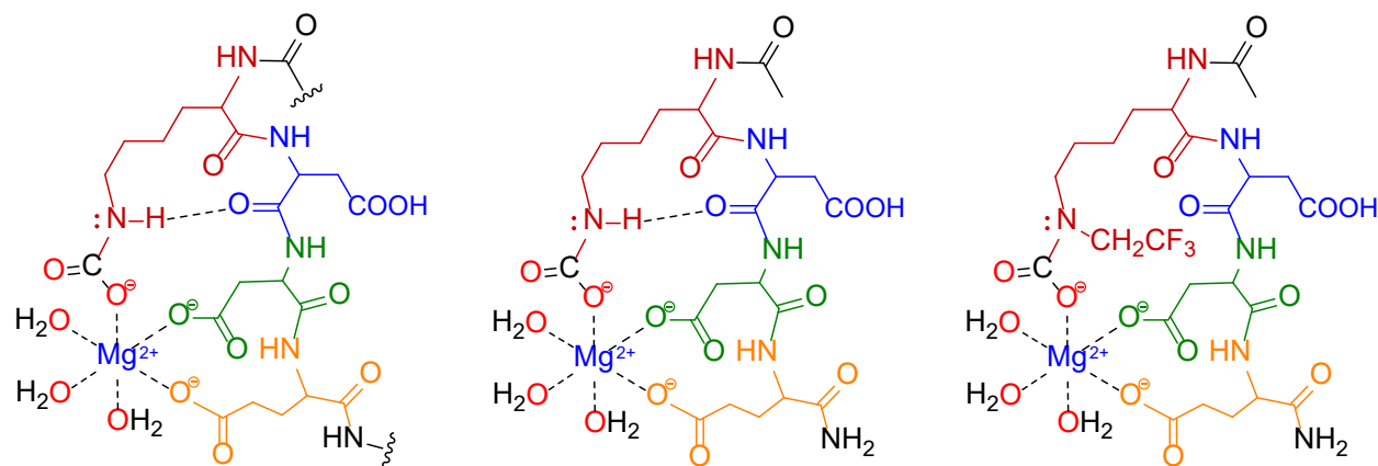
Scheme 1. The Lys-Asp-Asp-Glu sequence in the active site of RuBisCO (left), the capped KDDE tetramer (middle), and the capped tF KDDE tetramer with the fluorinated unnatural lysine tF K (right).
