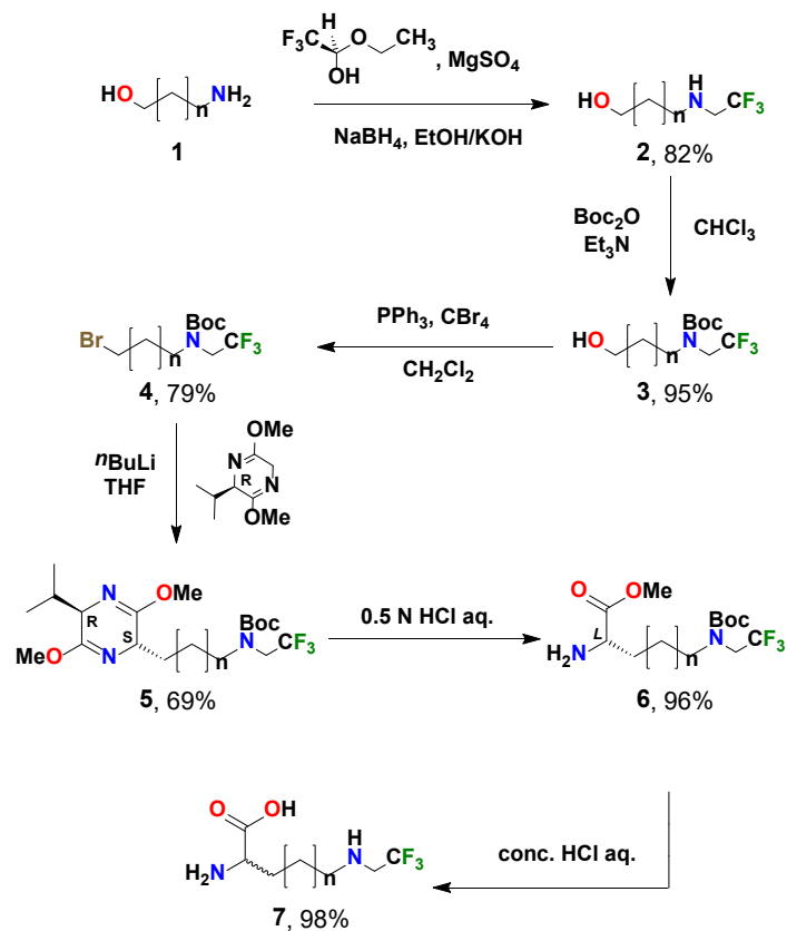
Scheme 2. Synthesis of N -trifluoroethyl substituted lysine analogs.
