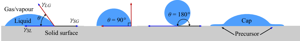
Figure 1. A schematic showing the equilibrium contact angle (i.e. \theta \equiv \theta_{eq} ), the surface tensions ( \gamma ), the threshold between low- and high-wetting regimes ( \theta_{eq} = 90^\circ ), and a situation of a non-wetting droplet ( \theta_{eq} = 180^\circ ). The last image demonstrates the occurrence of a precursor that is observed in some cases. In that case, the (macroscopic) contact angle is defined using the macroscopic part of the droplet, the cap in the rightmost image. The height of the precursor is in the molecular length scales (Hardy 1919; Nieminen et al. 1992; Popescu et al. 2012).
