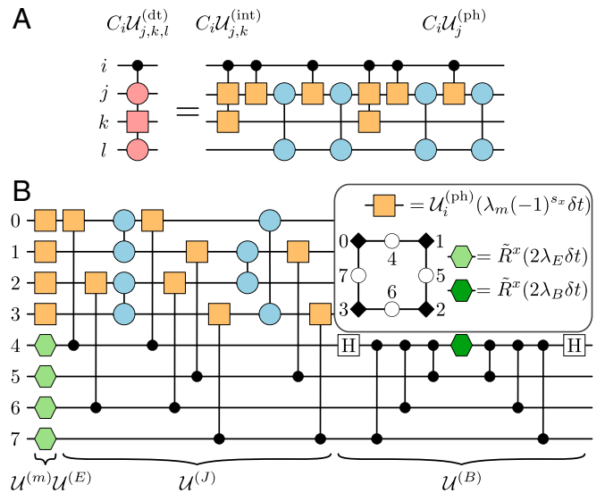
Fig. 5. Fermion-qubit quantum circuits. (A) Decomposition of C_i\mathcal{U}_{j,k,l}^{(\text{dt})}(\theta_1, \theta_2) , a density-dependent fermionic hopping controlled by ancillary qubit ( i ) into fermionic gates and the three-body fermion-qubit gate C_i\mathcal{U}_{j,k}^{(\text{int})} . The angles of the interaction and the controlled interaction gate are \pi . The angles of the first and third tunneling gates are (\theta_1, \theta_2, 0) , while for the second and fourth are (\theta_1, -\theta_2, 0) . (B) Trotter step required to time-evolve one plaquette under the \mathbb{Z}_2 LGT Hamiltonian Eq. 12, where atoms 0 to 4 and 5 to 7 encode local matter and gauge fields, respectively. The unitary circuits \mathcal{U}^{(p)} , with p \in \{m, E, J, B\} , implement the exponential of each term in the Hamiltonian, and the single-qubit rotations are given by \tilde{R}^x(\theta) = e^{-i(\theta/2)\sigma^x} (green hexagons) acting on the (|\tilde{1}\rangle, |1\rangle) subspace, while \mathcal{U}_i^{(\text{ph})}(\theta) = e^{-i\theta n_i} (orange box) is a local phase shift if a particle is present in tweezer i . We further use standard notations for qubit operations, namely, H indicates a Hadamard gate H = (-|1\rangle + |\tilde{1}\rangle)(1/\sqrt{2} + (|1\rangle + |\tilde{1}\rangle)(\tilde{1}/\sqrt{2}) , a dot denotes a control on the state |1\rangle , and two connected dots correspond to a CZ gate. The angles of the interaction gates are \pi , whereas the angles of the tunneling gates are (\lambda_j\delta t, 0, 0) .
