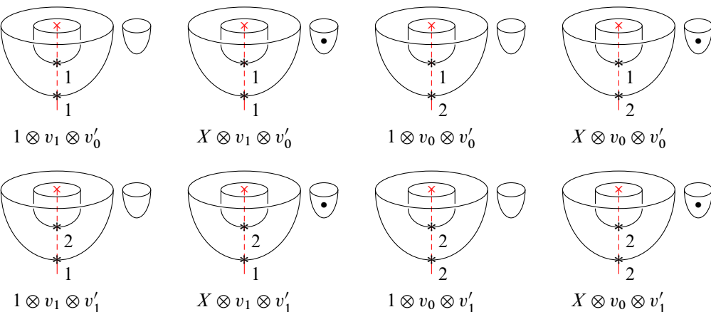
Figure 6: An example of the isomorphism \Phi_C when C consists of one contractible circle and two noncontractible circles. Basis elements \Sigma of \langle C \rangle are drawn with the corresponding basis element \Phi_C(\Sigma) \in \mathcal{G}_\alpha(C) written underneath.
