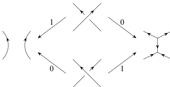
Figure 19: The 0- and 1-smoothings used to define the \mathrm{SL}(3) chain complex.
