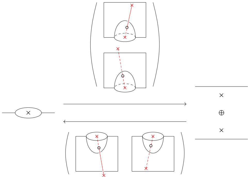
Figure 12: Isomorphisms which simplify a bigon region containing the puncture, for the theory \langle - \rangle_\circ . In the top map, the top foam has a type 1 point on the front half-bubble, and the bottom foam has a type 1 point on the back half-bubble. In the bottom map, the first foam has a type 1 point on the front half-bubble, and the second foam has a type 1 point on the back half-bubble.
