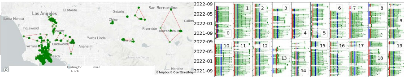
Fig. 4. Results of applying the second k-means model to a fleet of 20 trucks using data from July 2021 to August 2022. The 20 resulting clusters are represented by green dots and enclosed in red convex hulls. Additionally, a manual convex hull was assigned to the data to indicate the home base.
