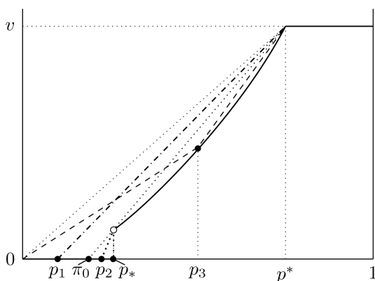
FIG. 7.—Optimal Poisson jump targets for different values of p . The solid curve represents the sender's value function in an SMPE with p_* and p^* .
