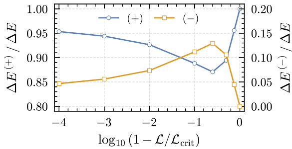
FIG. 7. Fraction of the total energy radiated by the polar and axial perturbations in the plunge process. We show both the polar [(+), left ordinate] and axial [−, right ordinate] total energies as functions of the particle’s angular momentum. The fraction of the total energy radiated via each radiative channel is nonmonotonic in \mathcal{L} , with the axial channel having a peak at \mathcal{L}/\mathcal{L}_{\text{crit}} \approx 0.75 . The polar contribution is at least \approx 85\% of the total energy budget for all values of \mathcal{L} considered.
