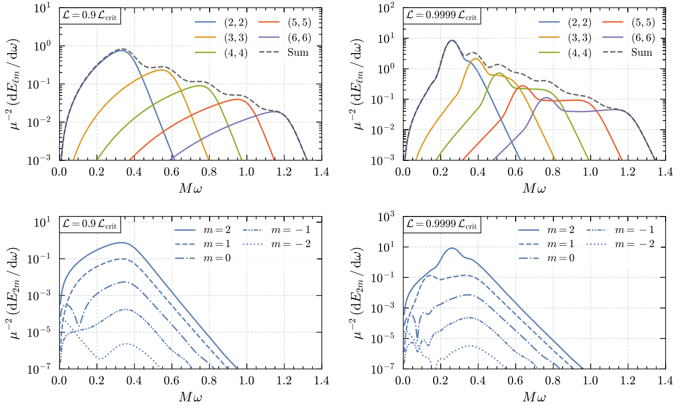
FIG. 5. The energy spectra for a particle plunging with angular momentum \mathcal{L} = 0.9\mathcal{L}_{\text{crit}} (left panels) and \mathcal{L} = 0.9999\mathcal{L}_{\text{crit}} (right panels) into a Schwarzschild black hole. Top panels: the energy spectra from the multipoles \ell = m from 2 to 6, (colored lines), and their sum (dashed line). Bottom panels: the energy spectra for the quadrupole perturbation \ell = 2 and all |m| \leq 2 in between. Note the different ranges in the ordinates across the panels. Our results agree with Ref. [29], which solved the Sasaki-Nakamura equation instead.
