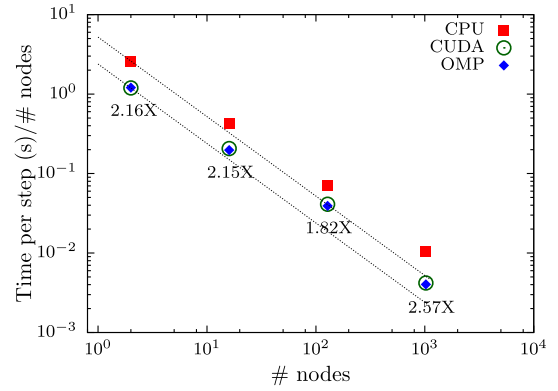
Fig. 8. Weak scaling performance of non-batched synchronous 3D FFT kernels on Summit. Performance of CUDA Fortran (green) and OpenMP (blue) versions are comparable. Speedup of OpenMP offload with respect to the CPU version is given as labels in the plot. Dashed lines indicate perfect weak scaling. (For interpretation of the references to color in this figure legend, the reader is referred to the web version of this article.)
