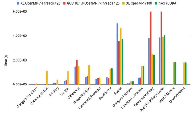
Fig. 4. Timings for computational kernels and data transfers in GENASIS BASICS RiemannProblem 3D with 256^3 cells for 50 cycles. CPU multithreading timings factored by 25X to fit plot. (For interpretation of the references to color in this figure legend, the reader is referred to the web version of this article.)
