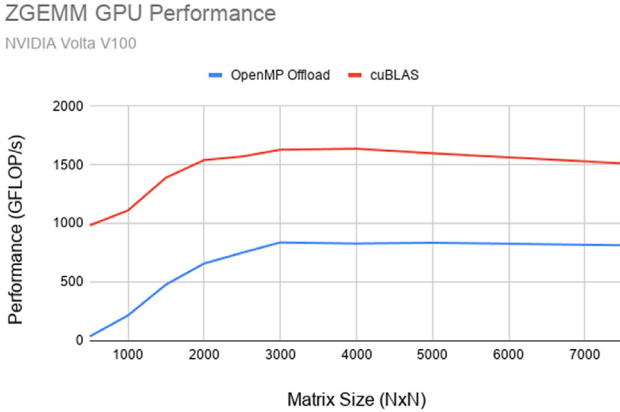
Fig. 13. Performance of selected BLAS routines implemented in FLENS using OpenMP offloading on a single Volta GPU versus cuBLAS performance.
