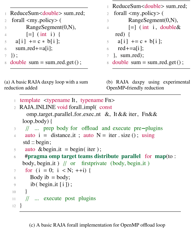
Fig. 19. Examples of RAJA usage and internals.
