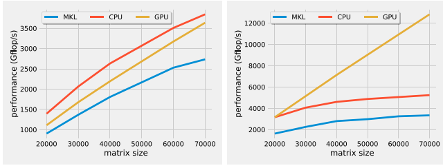
Fig. 18. Comparison of SLATE's performance on 4 nodes of the NERSC's supercomputer Cori against Intel's MKL ScaLAPACK implementation for LU factorization PDGETRF (left) and QR factorization PDGEQRF (right) in IEEE 64-bit floating-point precision.
