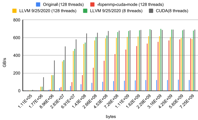
Fig. 10. Performance comparison of Benchmark_su3 in GridMini among different LLVM versions and CUDA. Results labeled Original and -fopenmp-cuda-mode used the LLVM GitHub version dated 07/31/2020, LLVM 09/25/2020 refers to the LLVM trunk version dated 09/25/2020, and CUDA uses cuda/10.1.243.
