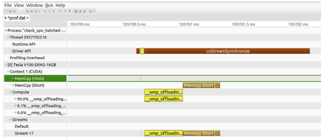
Fig. 15. Single OpenMP target offload region on a CUDA stream with minimal synchronization.
