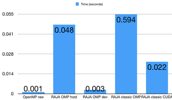
Fig. 20. Comparing reduction approaches on host and device with OpenMP.
