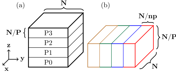
Fig. 6. Left: Decomposition of an N^3 solution domain among P MPI processes into slabs of data of size N \times N \times N/P . Right: Further decomposition of a slab into np smaller sub-volumes, each of size N \times N/np \times N/P .
