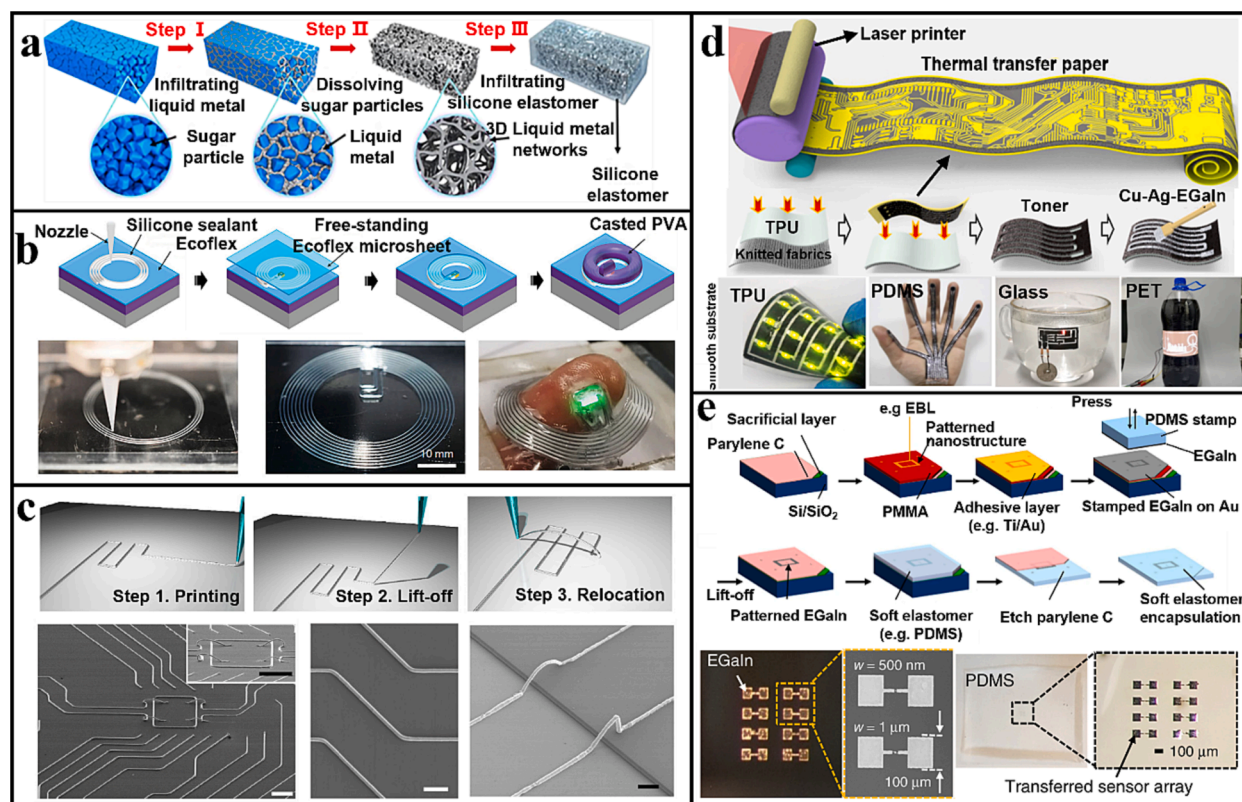
Fig. 4. Patterning of pristine LMs (a) The fabrication process of 3D LM structures by vacuum-assisted infiltration: (1) vacuum-assisted infiltration of LMs into a dissolvable porous template made of sugar particles, (2) dissolving the sugar template in an ice water bath to keep the 3D LM network in the solid state, and (3) vacuum-assisted infiltration of Ecoflex precursors into the 3D LM network and subsequent curing of Ecoflex at 0°C. Reprinted with permission from [8]. Copyright 2020 WILEY-VCH Verlag GmbH & Co. KGaA, Weinheim. (b) Schematic showing direct-print ultrathin microchannels for the injection of LMs (top panel). A PVA layer coated on the microchannel as the reinforcing support layer facilitates the injection process. The bottom panel shows the experimental setup of the 3D printing process (left), the as-fabricated ultrathin LM device in the free state (middle), or on the curvy tissue (right). Reprinted with permission from [9]. Copyright 2021 Wiley-VCH GmbH. (c) Direct 3D printing of LMs to form high-precision 3D structures through printing, lifting-off, and relocating (top), with the SEM image of 2D and 3D EGaIn patterns shown at the bottom. Scale bar: 10 \mu\text{m} . Reprinted with permission from [10]. Copyright 2019, The Authors. (d) High-yield patterning of Cu-Ag-EGaIn paste on a TPU substrate modified by toner for integrated devices (top). The fabrication process of Cu-Ag-EGaIn patterns starts with laser printing of toner patterns on a thermal transfer paper, followed by transferring to a TPU receiving substrate. Brush-coating the Cu-Ag-EGaIn paste on the TPU substrate forms the reserved image due to the low adhesion between the paste and toner. The bottom panel shows the optical image of the Cu-Ag-EGaIn-based integrated device upon bending deformations or on various curvy surfaces. Reprinted with permission from [11]. Copyright 2022 American Chemical Society. (e) Ultra-high precision LM patterns fabricated by using a metal seed layer defined by electron beam lithography (EBL). The fabrication process starts with coating the PMMA layer on the parylene-C/PAA layer, followed by the EBL patterning of PMMA. After the deposition of a metal layer on the PMMA layer, LMs are coated on the metal by using a PDMS stamp. The stamped LM/Au is patterned by a PMMA lift-off process and then coated with PDMS. After dissolving the PPA layer in water and plasma-etching of parylene-C, the LM pattern transferred to PDMS is encapsulated by another thin layer of PDMS to complete the fabrication process. The bottom panel shows the as-fabricated LM patterns on the donor substrate or the stretchable receiving PDMS substrate. Reprinted with permission from [12]. Copyright 2020, The Authors.
