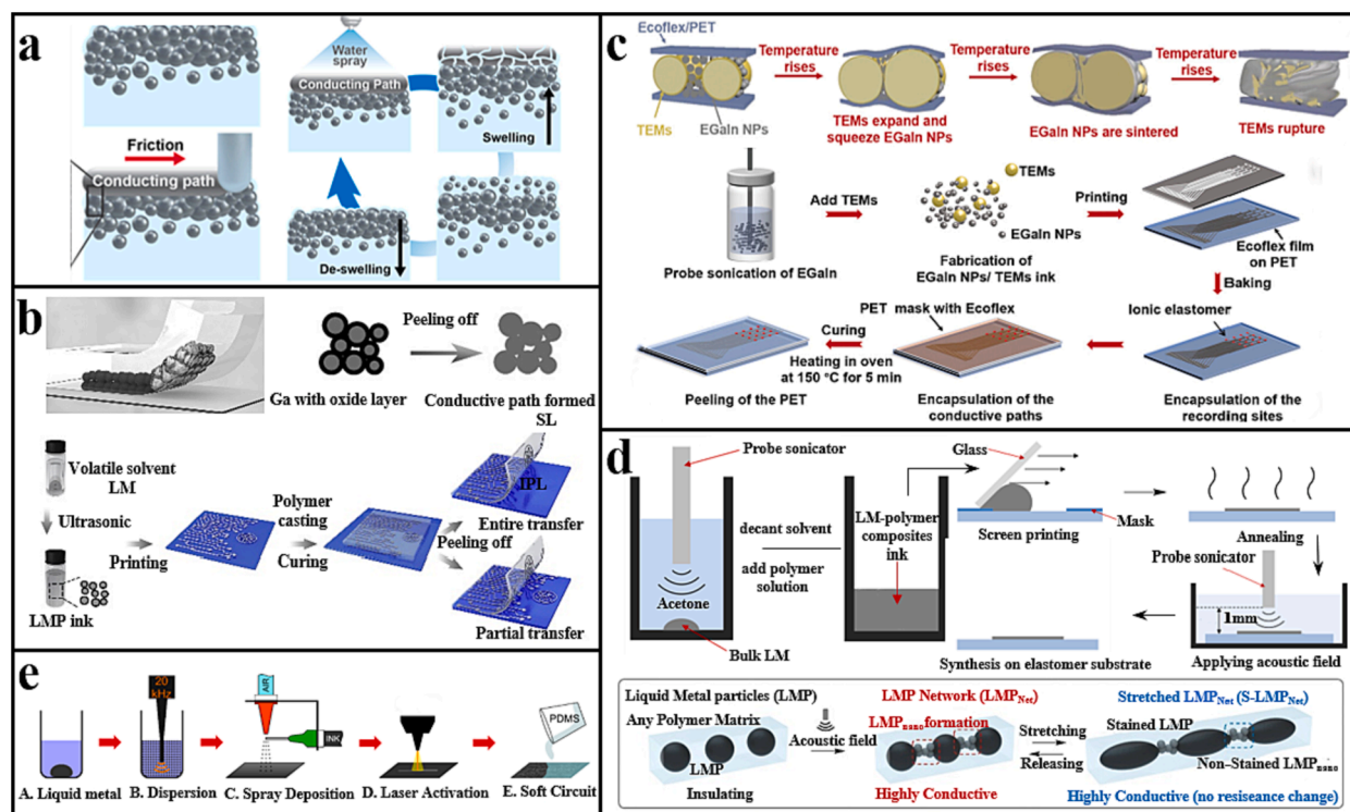
Fig. 5. Patterning of LMPs. (a) The mechanical sintering and erasing process of LMPs in a poly(ethylene glycol) diacrylate(PEGDA) hydrogel. Mechanical loading above the yield stress of \text{Ga}_2\text{O}_3 ruptures the oxide layer, leading to the formation of conductive pathways. The conductive LM pattern can be erased by water spray to swell PEGDA for the rewriting process. Reprinted with permission from [13]. Copyright 2019 American Chemical Society. (b) LMPs transferred to stretchable substrates are electrically activated due to the tensile stress from peel-off. LMPs in a volatile solvent (n-decyl alcohol) can be printed on the initial patterning layer (IPL) due to the improved wettability. After the evaporation of the volatile solvent, the curable polymer precursor is cast onto the stacked particles as the stripping layer (SL), which is peeled off from the IPL after curing. The entire or partial transfer of LMPs can be tuned by adjusting the affinity between the IPL and SL. Reprinted with permission from [14]. Copyright 2018, The Authors. (c) Thermal sintering of LMPs by utilizing thermal expansion microspheres (TEMs) in the LMP ink. The top panel shows the working principle of thermal sintering of LMPs. The oxide layer of LMPs ruptures to form interconnected conductive pathways at elevated temperatures due to the compressive stress from the thermal expansion of TEMs. The bottom pattern details the fabrication process of an LM-based biopotential sensing patch based on the thermal-activated LMP/TEM ink. The LMP/TEM prepared by tip sonication is patterned on an Ecoflex substrate by screen printing. After applying a protective layer on the recording site and an encapsulation layer on the interconnect, the biopotential sensing patch is activated by heating at 150^\circ\text{C} for 5 min. Reprinted with permission from [15]. Copyright 2023 Wiley-VCH GmbH. (d) Electrical activation of LMPs in an LMP/PU composite by the acoustic field (top). The fabrication of LM patterns starts with the screen-printing of the LMP/PU ink on an elastomeric substrate. After curing, the printed LM pattern is activated by a tip sonicator in a water bath. The bottom panel illustrates the mechanism of the acoustic activation process that relies on the formation of nano-sized LMPs between large LMPs. The small interspacing between nano-sized LMPs permits electron hooping and contributes to the conductive pathway. Upon stretching, the large LMP changes from spherical to ellipsoidal shape to release the local strain, while the shape of nano-sized LMPs and the spacing remain unchanged, leading to a strain-resilience electromechanical property. Reprinted with permission from [16]. Copyright 2022, The Authors. (e) Laser sintering of LMPs to form conductive patterns. The LMP dispersion in ethanol is air-sprayed on an elastomeric substrate, followed by laser-patterning with optimized working parameters. The thermal expansion of the LMP inner core of LMPs from the photothermal effect ruptures the oxide layer and forms conductive patterns. The region without laser scribing remains insulating. Reprinted with permission from [17]. Copyright 2018 American Chemical Society.
