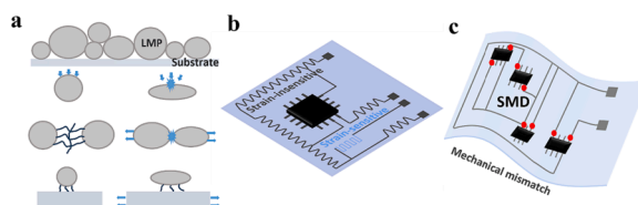
Fig. 12. Highly permeable LM-based electronics (a) High-resolution LM patterning involves the issues of yield strength, mechanical sintering, and interacting with supporting substrates of LMPs in submicron scale. (b) Schematic showing All-LM-based stretchable electronics with spatially dependent electromechanical properties (i.e., strain-insensitive and strain-sensitive). (c) LM-based integrated stretchable electronics with surface mountable devices (SMDs).
