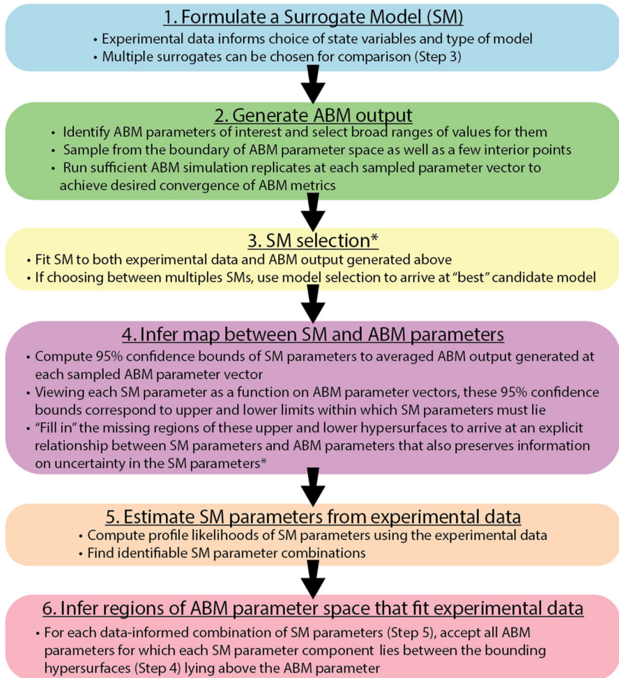
Fig. 2 Flowchart of the SMORe ParS algorithm
