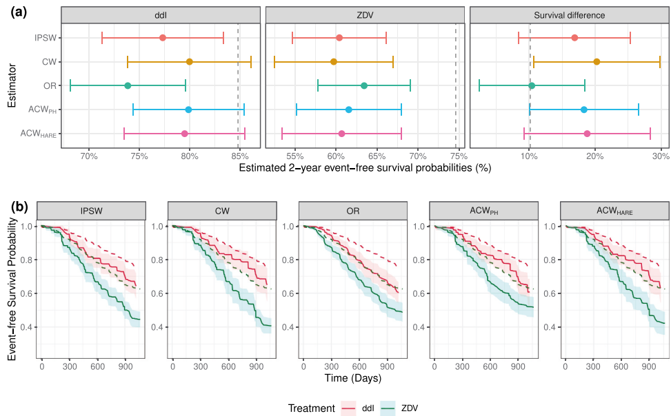
Figure B5. Estimated treatment-specific event-free survival probabilities in Thailand HIV patients for ddl vs. ZDV; (a) 2-year event-free survival probabilities; (b) treatment-specific survival curves. Dashed lines indicate the estimates from the RCT PH model.
