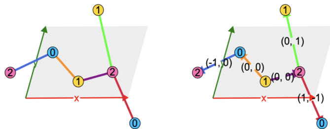
Figure 3 An undirected span-graph (left) and the (directed) shift-span-graph (right) of the periodic graph from Fig. 2 (middle). The pair of integers on a directed edge representative indicates the shift of the head-vertex; the tail of the edge representative is always chosen to be in the unit cell.
