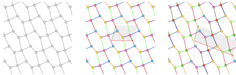
Figure 2 (Left) A 2D crystal. (Middle and right) Two of its possible periodic graphs. The highlighted unit cells represent the periodicity groups, and vertices or edges in the same orbit get identical colors.
