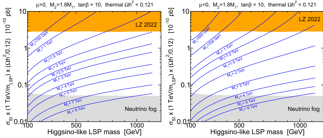
FIG. 2. The spin-independent LSP-nucleon cross section, scaled by factors of (1 \text{ TeV}/M_{\tilde{N}_1}) and \Omega h^2/0.12 , as a function of the Higgsino-like LSP mass M_{\tilde{N}_1} (related and comparable to |\mu| ), for various values of the Lagrangian parameter M_1 , as labeled. The wino mass parameter is taken to be M_2 = 1.8M_1 , as motivated by models with gaugino mass unification, and \tan\beta = 10 . The masses of the squarks, sleptons, and gluino, and the heavy Higgs bosons A, H, H^\pm are all set to 10 TeV, and M_h = 125.1 \text{ GeV} is imposed. The left panel shows results for \mu > 0 , and the right panel for \mu < 0 . The extent of the curves in the horizontal direction is set by the requirement \Omega h^2 < 0.121 . The (orange) shaded band at the top is the limit set by LZ 2022 [54]. The (gray) shaded band at the bottom is the expected neutrino fog level as defined in [74].
