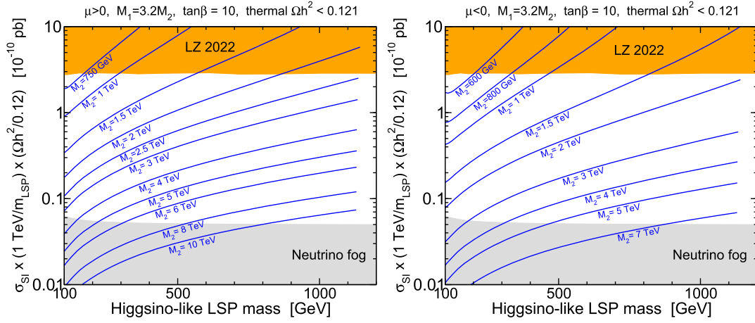
FIG. 3. The spin-independent LSP-nucleon cross section, scaled by factors of (1 \text{ TeV}/M_{\tilde{N}_1}) and \Omega h^2/0.12 , as a function of the Higgsino-like LSP mass M_{\tilde{N}_1} (related and comparable to |\mu| ), for various values of the Lagrangian parameter M_2 , as labeled. The bino mass parameter is taken to be M_1 = 3.2M_2 , as motivated by AMSB models, and \tan\beta = 10 . The masses of the squarks, sleptons, and gluino, and the heavy Higgs bosons A, H, H^\pm are all set to 10 TeV, and M_h = 125.1 \text{ GeV} is imposed. The left panel shows results for \mu > 0 , and the right panel for \mu < 0 . The extent of the curves in the horizontal direction is set by the requirement \Omega h^2 < 0.121 . The (orange) shaded band at the top is the limit set by LZ 2022 [54]. The (gray) shaded band at the bottom is the expected neutrino fog level as defined in [74].
