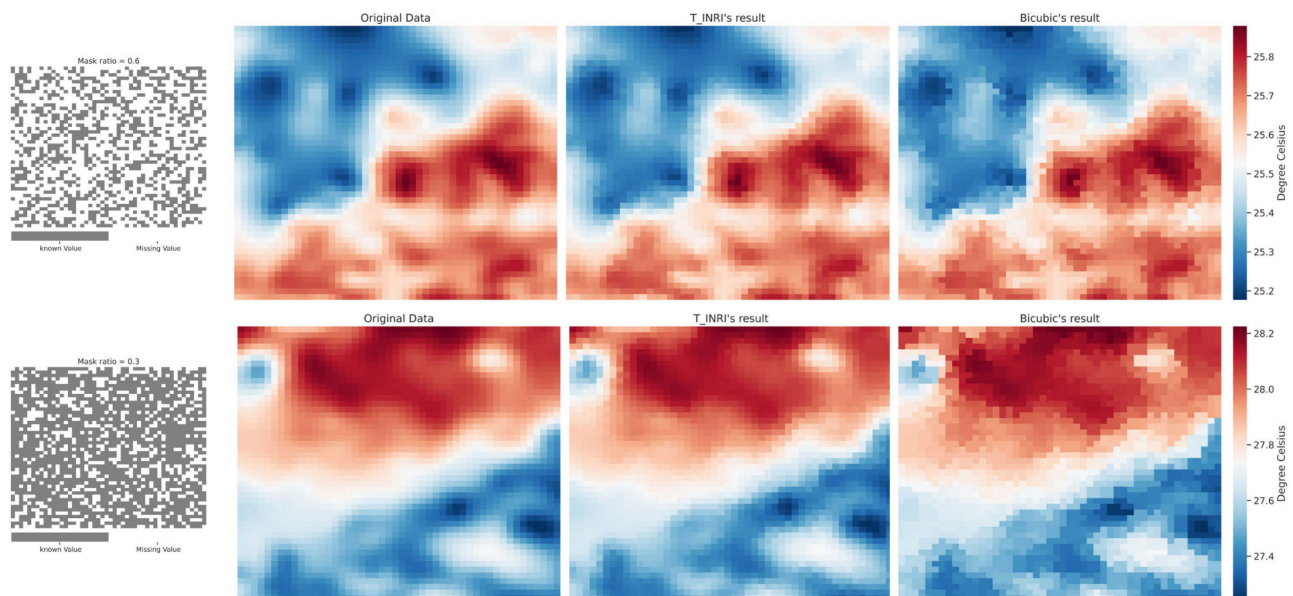
Figure 10. Visualization of the original data and results obtained by the proposed interpolation method and bicubic interpolation under different missing ratios. When the ratio is 0.3, the RMSE of the sample for T\_INRI is 0.008, and for the bicubic is 0.014; when the ratio is 0.6, the RMSE of the sample for T\_INRI is 0.015, and for the bicubic is 0.027.
