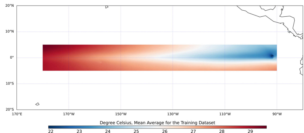
Figure 1. Region of SST data retrieval for the study area.
