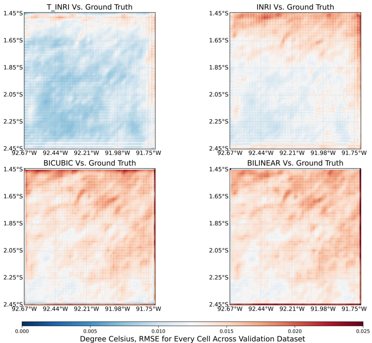
Figure 5. Qualitative comparison of generated HR SST data from different models. RMSE is calculated for every cell across validation dataset. The enhancement scale is \times 2 .
