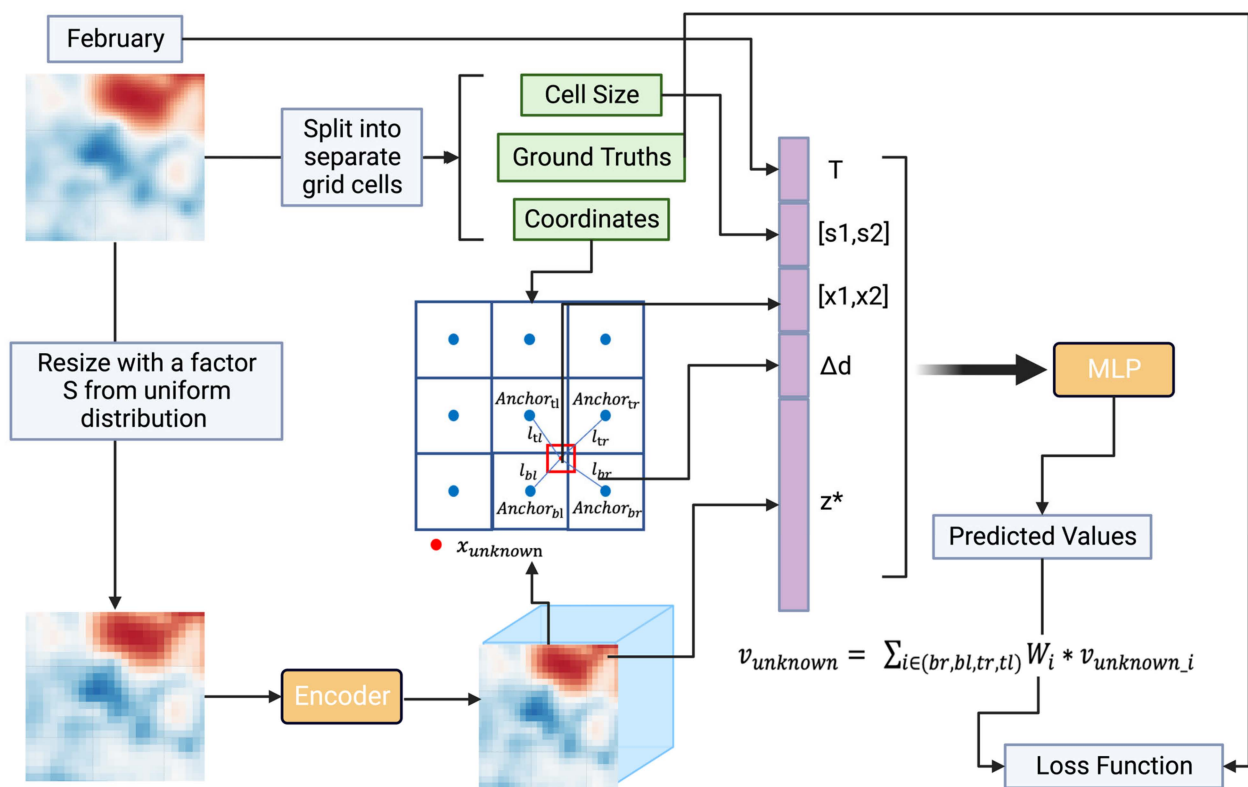
Figure 4. Workflow and training steps of the proposed interpolation method.
