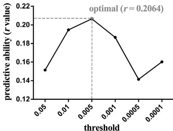
Figure 2. Optimal threshold for predictive model. r value = correlation between observed and predicted CA_r scores in combined network. CA_r , CA score after ruling out the effects of NAC items.
