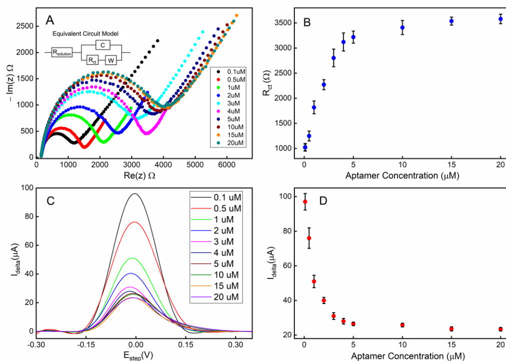
Figure 4. Electrode surface coverage characterization via electrochemical impedance spectroscopy (EIS) and square-wave voltammetry (SWV): (A) the Nyquist plot for the electrode when different concentrations of aptamers were used during the immobilization step; (B) the calibration curve corresponding to the Nyquist plot; (C) the SWV plot of the electrode when different concentrations of aptamers were used; (D) the calibration curve corresponding to the SWV plot. All error bars indicate 1 standard deviation ( n = 3 ).
