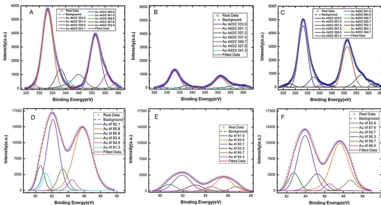
Figure 2. XPS spectra of the Au4d 3/2 peaks for (A) the bare gold electrode, (B) the electrode after aptamer immobilization, and (C) the aptamer-modified electrode after serotonin (5-HT) exposure. The XPS spectra for the Au4f peaks are also shown for (D) the bare electrode, (E) after aptamer immobilization, and (F) after serotonin 5-HT exposure to the modified electrode.
