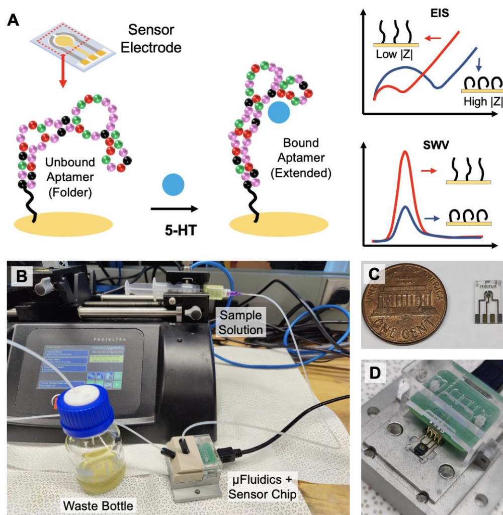
Figure 1. Overview of the aptamer-based electrochemical serotonin sensing: (A) serotonin-binding aptamers immobilized on the electrode undergo conformational change from folded to extended upon target recognition. EIS and SWV techniques can be applied for serotonin quantification; (B) for continuous real-time monitoring, the sample buffer solution is injected with a syringe pump into the microfluidic device containing the sensor chip; (C) image of the 3-electrode sensor chip; (D) the electrodes on the chip are securely connected to the terminals of the potentiostat via spring-loaded pins.
