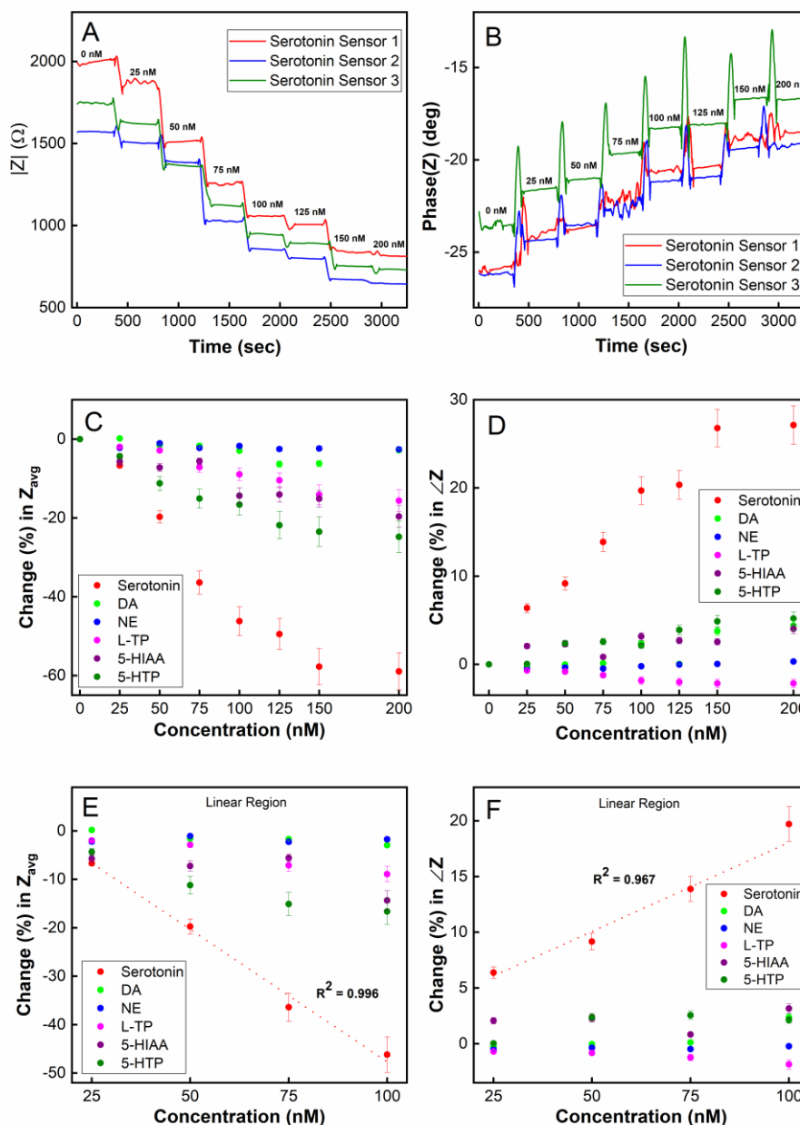
Figure 6. Real-time detection of serotonin (5-HT) using single-frequency EIS (SF-EIS): (A) plot of impedance magnitude ( |Z| ) vs. time; (B) plot of impedance phase ( \angle Z ) vs. time; (C) target selectivity test in a real-time sensing mode using averaged |Z| ( Z_{avg} ) as a sensor readout; (D) target selectivity test in real-time using \angle Z as a sensor readout; a linear detection range of 25–100 nM was observed using (E) the impedance magnitude ( |Z| ) and (F) the impedance phase ( \angle Z ).
