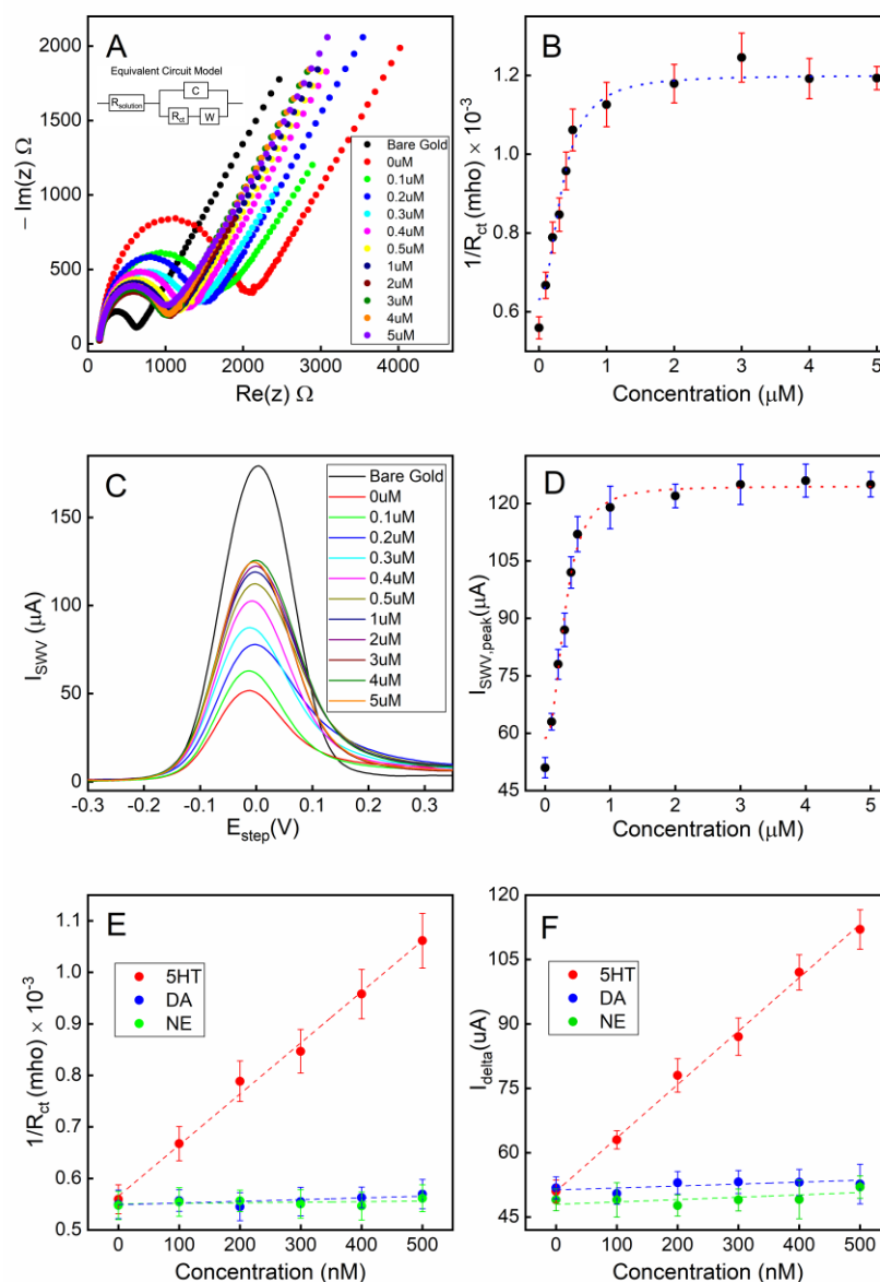
Figure 5. Detection of serotonin (5-HT) under a static fluidic environment: (A) Nyquist plots of EIS under various concentrations of serotonin (5-HT) exposed to the sensor; (B) a calibration curve showing the conductance vs. serotonin (5-HT) concentration; (C) SWV responses of the sensor to various concentrations of serotonin (5-HT); (D) a calibration curve showing the peak current of the SWV curve vs. serotonin (5-HT) concentration; (E) a calibration curve for EIS-based sensing in the linear range; (F) a calibration curve for SWV-based sensing in the linear range. All error bars indicate 1 standard deviation ( n = 3 ).
