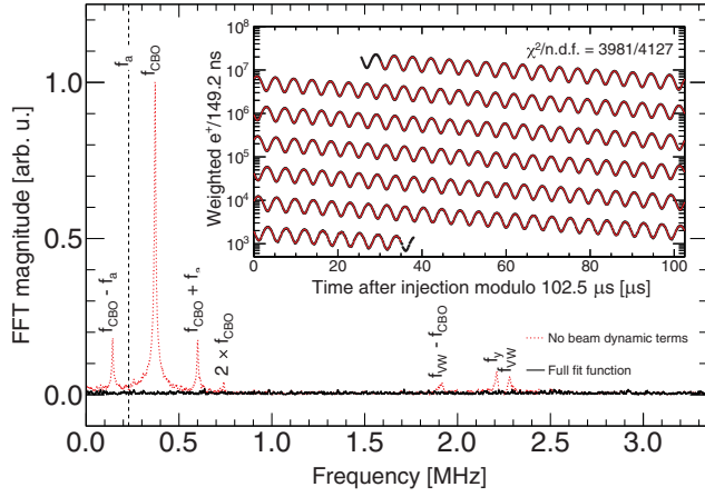
FIG. 1. Fourier transform of the residuals from a fit following Eq. (3) excluding \eta_N , \eta_A , and \eta_\phi (red dashed line), and from the full fit (black line). The peaks correspond to the missing betatron frequencies and muon losses. Data are from the Run-3a data set. Inset: corresponding asymmetry-weighted e^+ time spectrum (black line) with the full fit function (red line) overlaid.
