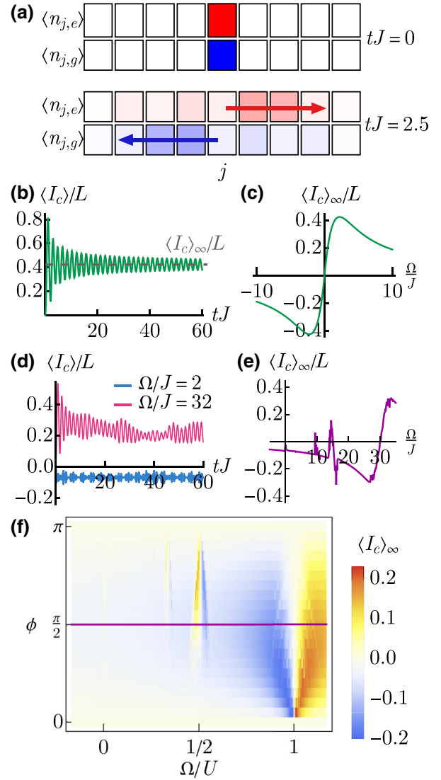
FIG. 2. (a) Time-evolution snapshots of populations \langle \hat{n}_{j,e} \rangle , \langle \hat{n}_{j,g} \rangle for a single-atom initial state |\psi_0\rangle_{\text{1atom}} = (1/\sqrt{2})(\hat{c}_{j=0,e}^{\dagger} + \hat{c}_{j=0,g}^{\dagger})|0\rangle in the gauged frame. The parameters are \Omega/J = 2 and \phi = \pi/2 . (b) Evolution of the chiral current for a noninteracting system U = 0 with flux \phi = \pi/2 , drive \Omega/J = 2 , and system size L \rightarrow \infty . (c) Long-time average current in terms of \Omega/J for the noninteracting system using the same flux. The analytic expression is given in Eq. (15). (d) Evolution of the chiral current for a strongly interacting system U/J = 30 with flux \phi = \pi/2 and drive strengths \Omega/J = 2, 32 . System size is L = 9 . (e) Average current for the interacting system with varying \Omega/J , averaging over tJ = 0 to 500. (f) Average current for the strongly interacting system across the parameter space of \Omega/U and \phi . The violet line corresponds to panel (e).
