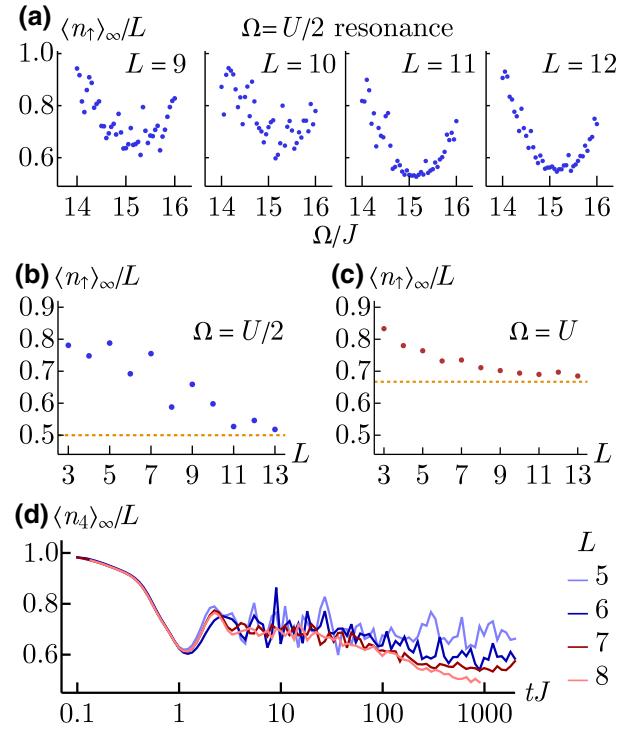
FIG. 13. (a) Long-time average population \langle \hat{n}_\uparrow \rangle_\infty for the n = 2 system near the \Omega = U/2 resonance, for different system sizes L . The parameters are U/J = 30 , \phi = \pi/2 , time evolution is done to tJ = 1500 , and averaging is done over the second half of the evolution, tJ = 750 to 1500 . (b) Long-time average population at the \Omega = U/2 resonance in terms of system size, fixing \Omega/J = 15.15 (where the peak appears to be centered). The orange dashed line is the thermal prediction of 1/2 . (c) Same as (b) but for the \Omega = U resonance, fixing \Omega/J = 30.15 . (d) Long-time average population for the n = 4 system at the \Omega = U/2 resonance for different system sizes L . The parameters are U/J = 30 , \phi = 2.0 .
