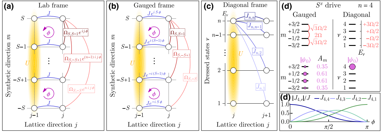
FIG. 5. (a) Schematic of the n > 2 system now engineering an n -leg ladder in the lab frame. The synthetic dimension states are indexed m \in \{-S, -S+1, \dots, S\} with S = (n-1)/2 the size of an effective onsite spin. Motion along the synthetic direction is induced by a laser with couplings \Omega_{m,m'} between internal states m, m' and a phase e^{ij(m-m')\phi} to emulate the magnetic field. Only the couplings from the m = S state to the others are shown for simplicity, although generically each spin state can be coupled to each other. The SU(n) symmetric interactions are all to all in the synthetic dimension and onsite in the lattice dimension. (b) Visualization of the same system in the gauged frame where the flux is put into the tunneling terms. (c) Visualization of the system in the diagonal frame, where the synthetic spin dimension is comprised of dressed spin states \nu \in \{1, \dots, n\} that are single-particle eigenstates of the drive. In this frame the nearest-neighbor tunneling can flip spin from \nu to \nu' with corresponding matrix element J_{\nu,\nu'} . Again, only couplings from \nu = n are shown for simplicity, although all dressed states generically couple to all others. (d) Couplings between spin states in the gauged frame and corresponding dressed energy levels in the diagonal frame for a \hat{S}^x -type drive and n = 4 states. The typical initial state of all atoms in the highest-energy dressed state \nu = 4 is shown in both frames with the corresponding wavefunction amplitude A_m of each spin state in the gauged frame. (e) Tunneling matrix elements J_{\nu,\nu'} allowed for the initially occupied dressed state \nu = 4 for the drive in panel (d).
