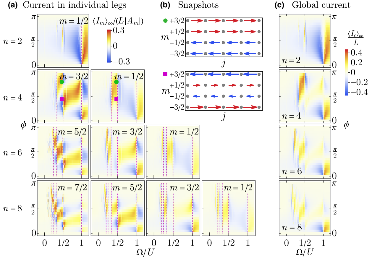
FIG. 6. (a) Average spin current in each leg m for different synthetic dimension sizes n across the parameter range of \Omega/U and \phi . We scale the current along leg m by the initial wavefunction probability amplitude |A_m| = |\langle \psi_0 | m \rangle| in that leg. Prominent resonant crossovers are highlighted with dashed lines. Only m > 0 legs are shown; the other legs are equal and opposite, \langle \hat{I}_m \rangle = -\langle \hat{I}_{-m} \rangle . The system size is L = 9, 5, 4, 4 for n = 2, 4, 6, 8 , respectively. Interactions are fixed at U/J = 30 . The system is evolved to time tJ = 500 before taking the average. (b) Snapshots of current profiles for the n = 4 system in two particular regions of parameter space indicated by the green and purple markers in panel (a). The size of the arrows is proportional to the scaled average current along that link; current across the periodic link is not shown. (c) Overall average chiral current obtained by summing over all legs (with no scaling factors) for the same parameters as (a).
