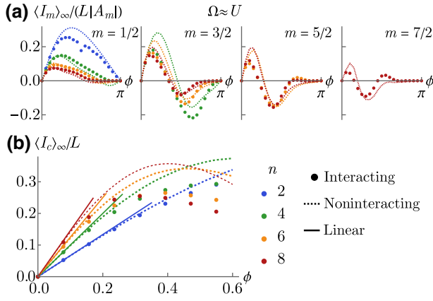
FIG. 7. (a) Average scaled current in different legs m close to the \Omega = U resonance for n = 2, 4, 6, 8 , fixing U/J = 30 and \Omega/J = 33 . The dots show the numerically computed data for the strongly interacting system, sizes L = 9, 5, 4 as before, evolved to time tJ = 500 . The dashed line is the corresponding average for a noninteracting system U = 0 with the same initial condition and effective drive strength \Omega/J = 3 , and the same distance from the \Omega = U resonance assuming that it is shifted from \Omega = U to \Omega = 0 . (b) Average chiral current for the same resonance in the \phi \ll 1 limit. The solid lines are a linear approximation with a slope given by Eq. (30).
