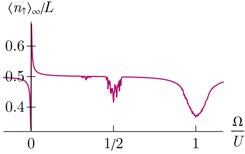
FIG. 14. Long-time average population \langle \hat{n}_\uparrow \rangle_\infty for the n = 2 system with the different initial state |\tilde{\psi}_0\rangle from Eq. (B2). The parameters are L = 9 , U/J = 30 , \phi = \pi/2 , and time averaging is done out to tJ = 500 .
