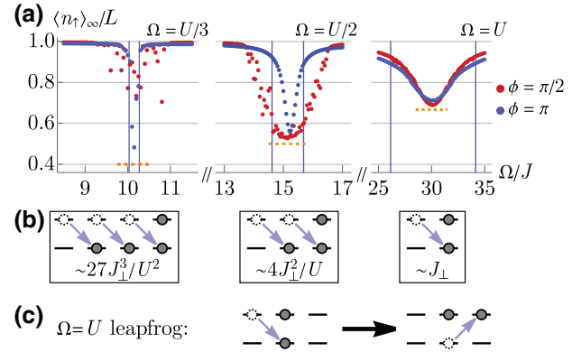
FIG. 4. (a) Long-time average of the population \langle \hat{n}_\uparrow \rangle near the resonances \Omega = U/3, U/2, U for different fluxes \phi = \pi/2, \pi . The system size is L = 11 and the interaction strength is U/J = 30 . Time evolution is done out to tJ = 1500 , and averaging is done over tJ = 750 to 1500 to avoid the initial population decay. The \phi = \pi resonance widths are set by the respective rates 27J_\perp^3/U^2, 4J_\perp^2/U, J_\perp ; the vertical blue lines represent values of \pm 4 times the corresponding rate for each resonance. The \phi = \pi/2 resonance widths are instead broadened by an effective bandwidth of about J_\parallel . Note that the specific positions of the resonances are also shifted due to off-resonant superexchange interactions by a factor of the order of about J^2/U . The orange dashed lines correspond to infinite-temperature thermal average predictions of 2/5, 1/2, and 2/3, respectively (see Appendix C). (b) Associated interaction-enabled tunneling processes for each respective resonance in (a). (c) Leapfrog process by which pairs of \uparrow atoms can move at the \Omega = U resonance via J_\perp only.
