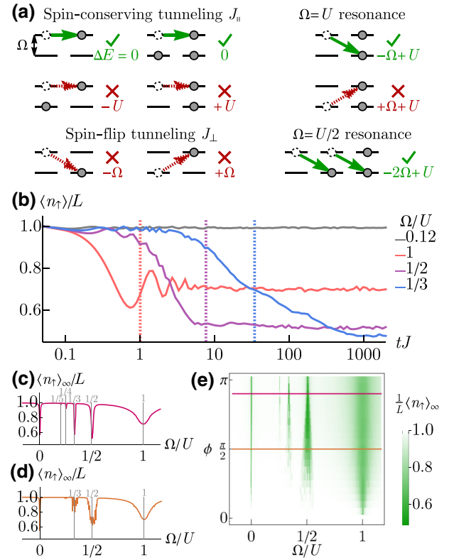
FIG. 3. (a) Diagrams of the allowed and forbidden tunneling processes of the n = 2 system in the diagonal frame for \Omega, U \gg J . The energy cost for an atom hopping from one level (indicated by an empty circle) to another (indicated by the arrow) is shown. Processes with green arrows cost zero energy and are allowed, while ones with red arrows are off-resonant and forbidden. Interaction-enabled tunneling processes are shown for the \Omega = U and \Omega = U/2 resonances, although higher-order ones can occur as well. (b) Time evolution of the dressed state population \langle \hat{n}_{\uparrow} \rangle for a quench starting with all atoms in that state, for a system size L = 11 , large flux \phi = 9\pi/10 , strong interactions U/J = 30 , and selected drive strengths \Omega/U = 0.12 (nonresonant) and \Omega/U = 1, 1/2, 1/3 (different resonances). For the latter, the associated timescales tJ_{\perp} = 1 , 4tJ_{\perp}^2/U = 1 , 27tJ_{\perp}^3/U^2 = 1 are indicated by vertical dotted lines. (c), (d) Long-time average of the population \langle \hat{n}_{\uparrow} \rangle_{\infty} with U/J = 30 , system size L = 9 , and flux values of (c) \phi = 9\pi/10 and (d) \phi = \pi/2 , averaging out to time tJ = 500 . Discernable resonances \Omega = U/q are labeled. (e) Average population across the parameter range of \Omega/U and \phi , still using U/J = 30 and L = 9 . The colored lines correspond to panels (c) and (d).
