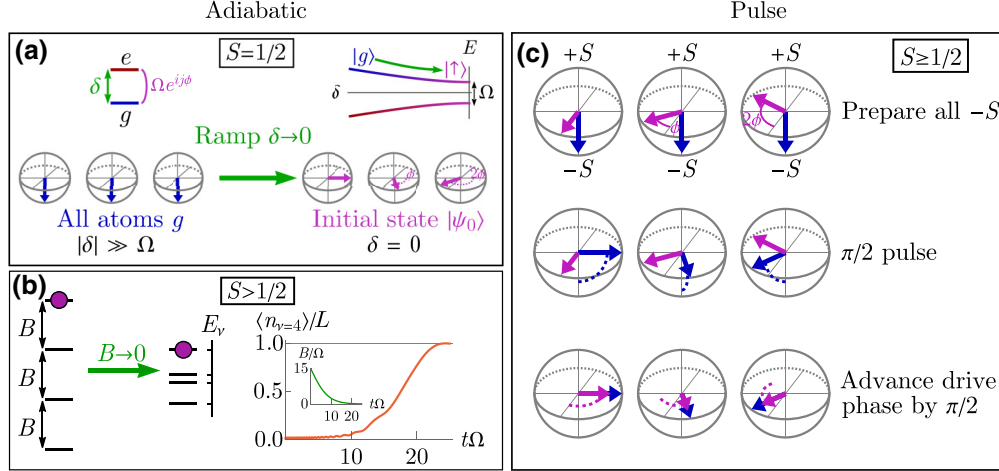
FIG. 11. (a) State preparation using a single-particle adiabatic ramp for n = 2 (spin S = 1/2 ). Atoms are initialized in the lab frame spin state g , and a laser coupling is turned on with a large negative detuning -\delta \gg \Omega . Ramping \delta \rightarrow 0 sweeps the system into the desired initial state |\psi_0\rangle with every lattice site in the highest-energy eigenstate \uparrow of the drive. (b) Similar adiabatic preparation for an n > 2 system ( S > 1/2 ). The detuning is replaced by, e.g., a magnetic field splitting of hyperfine states proportional to a field strength B , which is ramped to zero. The plot shows a numerical simulation of such a ramp for an n = 4 system, using the coupling scheme in Fig. 10(b) for sample parameters of \Omega^+/\Omega^0 = 3 , \Omega/J = 2 , and U/J = 30 . The inset shows the ramp profile. The highest-energy drive eigenstate v = 4 is prepared with > 99\% fidelity. (c) State preparation protocol using a pulse and phase skip sequence, which works for a system with a \hat{S}^x drive and any n \geq 2 . Blue arrows denote the spin direction of each atom, while purple arrows denote the laser drive direction. Atoms are first prepared in a single lab frame spin state m = -S without any detuning or field splitting. The laser drive is turned on and used to implement a \pi/2 pulse, rotating the spins onto the equator of the Bloch sphere (or the generalized Bloch sphere of the fully symmetric manifold for n > 2 ). The drive phase is then skipped ahead by \pi/2 with, e.g., a fast detuning pulse, which advances its axis of rotation to be aligned with the spin state. This prepares the desired |\psi_0\rangle .
