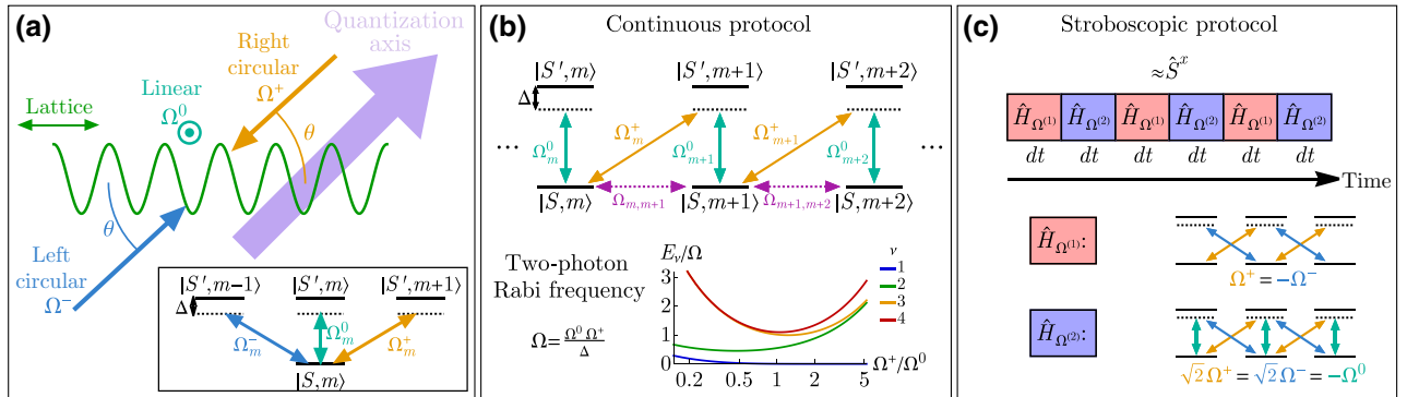
FIG. 10. (a) General schematic for realizing the SU(n) system using a Raman coupling in a lattice with alkaline-earth atoms. Far-detuned Raman beams with different polarizations illuminate the lattice. The one-photon couplings \Omega_m^0, \Omega_m^{\pm} are all m dependent due to Clebsch-Gordan coefficients, but proportional to overall magnitudes \Omega^0, \Omega^{\pm} . The linearly polarized \Omega^0 beam propagates perpendicular to the lattice direction, while the right- and left-circular beams \Omega^+, \Omega^- point in equal and opposite directions at an angle \theta to the lattice direction. (b) Protocol for generating a “nearest-neighbor” drive coupling along the synthetic dimension. The linear and right-circular beams are used to realize effective two-photon couplings \Omega_{m,m+1} . The overall intensity of the couplings is set by \Omega = \Omega^0 \Omega^+ / \Delta . The bottom plot shows the energies of the onsite drive eigenstates as a function of \Omega^+ / \Omega^0 , demonstrating that the dressed state spectrum can be tuned. (c) Protocol for generating a spin- S \hat{S}^x -type coupling. Two different laser configurations \hat{H}_{\Omega^{(1)}} and \hat{H}_{\Omega^{(2)}} are stroboscopically alternated. They realize effective drives of (\hat{S}^x)^2 and -(\hat{S}^x)^2 + \hat{S}^x , respectively, yielding the desired \hat{S}^x provided the stroboscopic rate is faster than the tunneling and interactions.
