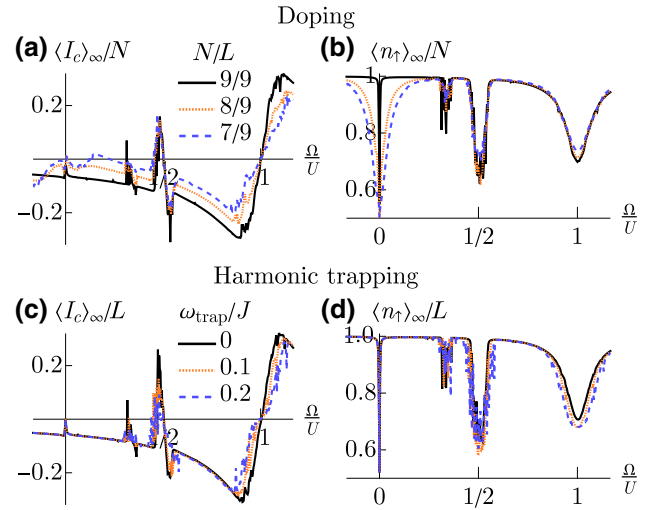
FIG. 12. (a) Average chiral current for the n = 2 system with holes in the initial state. The parameters are L = 9 , U/J = 30 , \phi = \pi/2 . Time averaging is done out to tJ = 500 . The N/L = 8/9 curves have a single hole initially at lattice site j = 1 , while the N/L = 7/9 curves have holes initially at sites j = 1, 3 . (b) Average dressed state population for the same setup. (c) Average chiral current for the n = 2 system in the presence of a harmonic trap \hat{H}_{\text{trap}} . We use the same parameters as (a), except with open boundaries and no holes. (d) Average dressed state population for the same setup.
