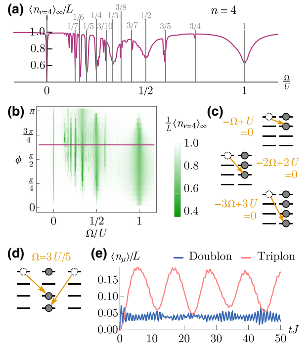
FIG. 8. (a) Long-time average population of the initially populated dressed state \langle \hat{n}_{v=4} \rangle_\infty for an n = 4 system as a function of \Omega/U . The interactions are fixed at U/J = 30 , the system size at L = 5 , and the flux at \phi = 2.0 [we use this flux rather than a simpler value like \pi/2 to avoid accidental cancellations of dressed tunneling matrix elements in Eq. (26)]. Resonances at \Omega = pU/q are labeled by their p/q values. (b) Long-time average population for the same system across the parameter space of \Omega/U and \phi . The purple line corresponds to panel (a). (c) Allowed spin-flip tunneling processes at the \Omega = U resonance. Doublons, triplons, and quadruplons can all be formed. (d) Two-step resonant process at the \Omega = 3U/5 resonance, forming a triplon. (e) Time evolution of fraction of lattice sites with exclusively two atoms (doublon) and three atoms (triplon) at the \Omega = 3U/5 resonance, for parameters L = 6 , U/J = 30 , \Omega/J = 18 .
