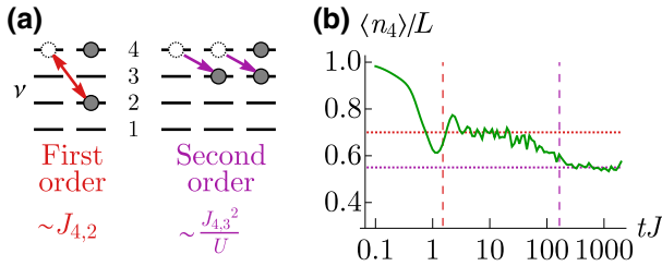
FIG. 9. (a) Dominant resonant processes for an n = 4 system at the \Omega = U/2 resonance for our initial state with all atoms in the highest-energy dressed state \nu = 4 . The typical rates for each process are shown. Other processes with similar rates can also occur, although they require additional moves to become allowed starting from this initial state. (b) Time evolution of the dressed state population. System size is L = 7 , parameters are U/J = 30 , \Omega/J = 15 , \phi = 2.0 . The system first saturates to an average of approximately 0.7 (dotted red line to guide the eye; not a theory prediction), which is close to the prediction of \frac{2}{3} from the first-order resonant process. At later times there is a further saturation to a different average of approximately 0.54 (dotted purple line to guide the eye). The associated timescales t|J_{4,2}| = 1 and t|J_{4,3}|^2/U = 1 are shown by the dashed red and purple lines, respectively.
