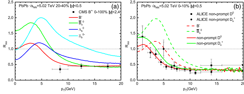
FIG. 4. (a) Nuclear modification factors for ground-state B^- , \bar{B}_s^0 , \Lambda_b^0 , and \Xi_b^{0,-} in 20%–40% \sqrt{s_{NN}} = 5.02 TeV PbPb collisions at midrapidity, together with CMS data for B^{+-} in 0%–100% centrality [72]. (b) The same for nonprompt D^0 and D_s^+ (0%–10% centrality) in comparison with ALICE data [83,84].
