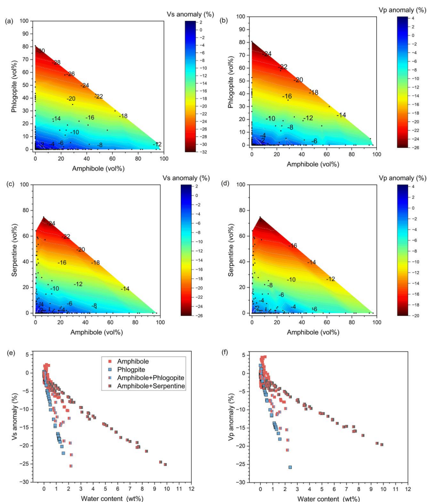
Figure 4. (a) Vs, and (b) Vp anomalies of metasomatized mantle rocks resulted from (co)existence of amphibole or phlogopite. (c) Vs, and (d) Vp anomalies of metasomatized mantle rocks resulted from (co)existence of amphibole or serpentine. (e) Vs, and (f) Vp anomalies of metasomatized mantle rocks as a function of bulk rock water content. In (a)–(d), the dots refer to Vp and Vs anomalies calculated from xenolith data in Table S4 of the Supporting Information S1, and the numbers refer to Vp and Vs anomalies along different contours.
