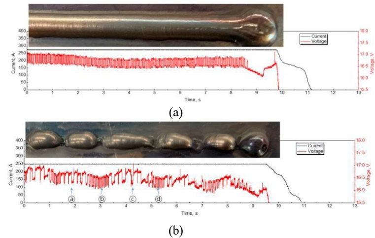
FIGURE 8: MACHINE LEARNING FOR REAL-TIME ANOMALY DETECTION (a) NORMAL AND (b) ABNORMAL BEADS [32]
