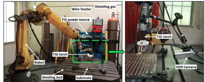
FIGURE 6: EXPERIMENTAL ENVIRONMENT INCLUDING WIRE FEEDER, SHIELDING GAS, TIG POWER SOURCE, TIG TORCH, ROBOT, AND HDR CAMERA
