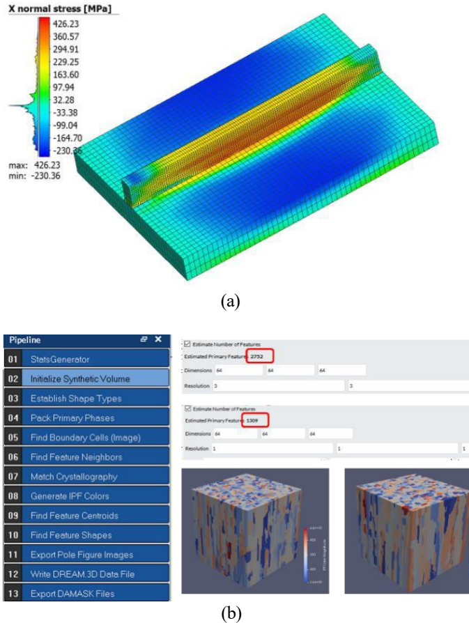
FIGURE 7: DT COMPONENTS FOR WAAM PARTS: (a) RESIDUAL STRESS AND (b) CPFEM
