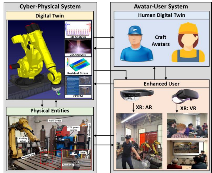
FIGURE 5: CONCEPTUAL ARCHITECTURE OF THE DH-SM FOR A WAAM CASE
