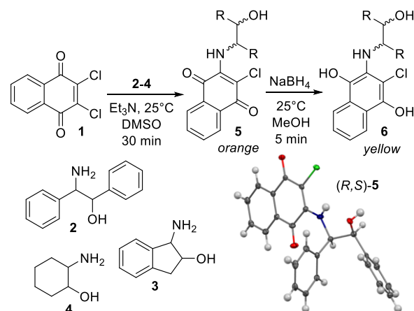
Scheme 1. Reaction of naphthoquinone 1 with amino alcohols 2-4 to 5 and reduction to the hydroquinone derivative 6 . The crystal structure shown is derived from the reaction between 1 and ( R,S )- 2 .
