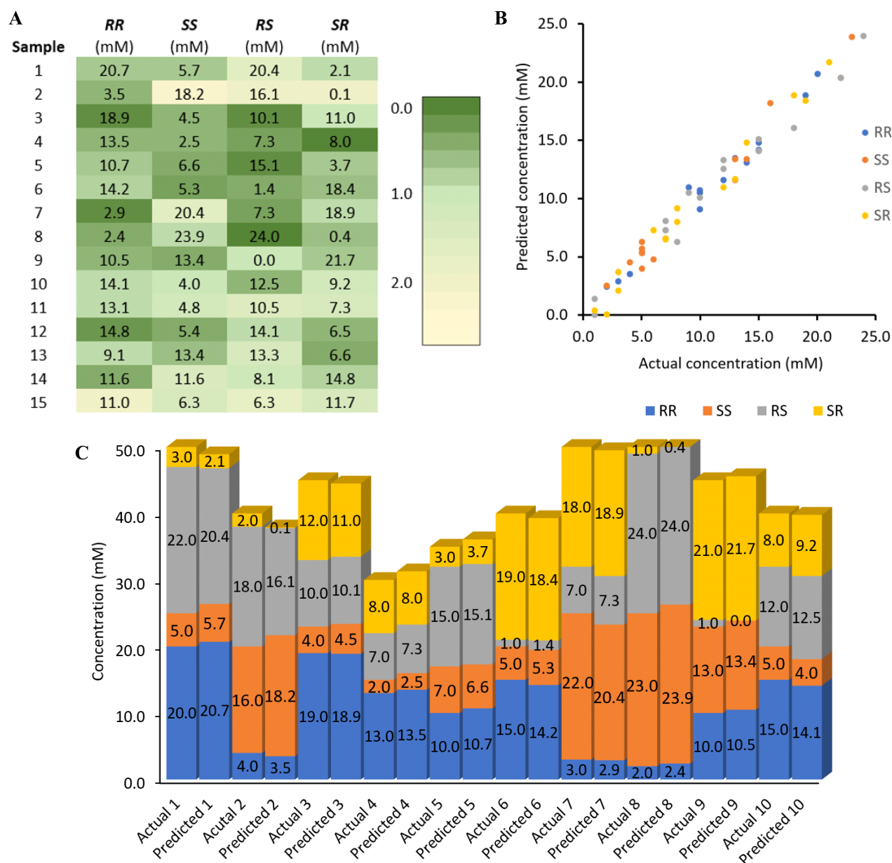
Figure 4. Heat map, plot of actual versus predicted stereoisomer concentrations, and bar chart of the first ten samples. A. The heatmap represents the absolute %error ranging from 0.0 (dark green) to the maximum of 2.2% (light yellow). B. Plot showing the consistently small assay inaccuracy and robustness over a 25 mM range for each stereoisomer. C. The bar chart compares the assay results together with the overall sample concentrations which was varied from 30.0 mM to 50.0 mM. The complete bar chart with all 15 samples can be found in the ESI.
