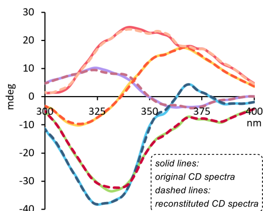
Figure 3. Reconstitution of CD spectral information obtained by sensing stereoisomeric mixtures of 2 with naphthoquinone 1 (oxidized state). See ESI for details.
