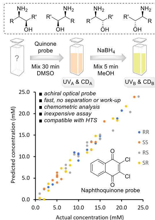
Figure 1. Chemometric Sensing of complicated stereoisomeric mixtures with a redox-responsive chirality probe.
