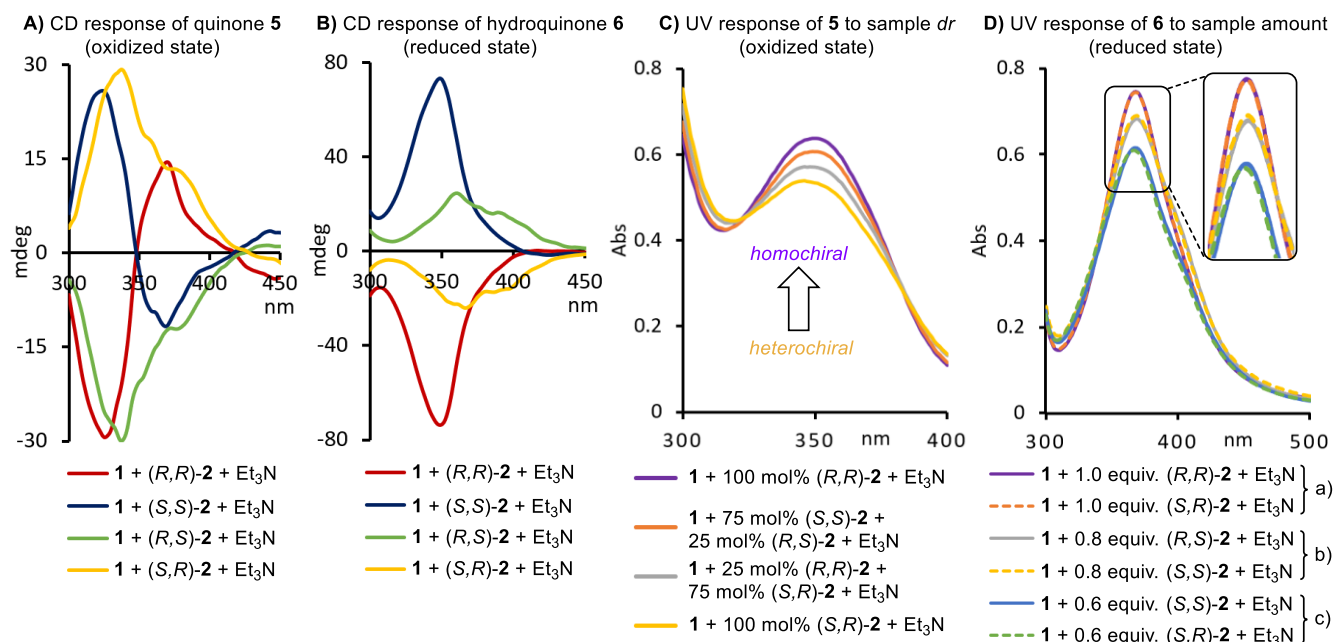
Figure 2. CD and UV responses of the quinone/hydroquinone redox couple derived from amino alcohol 2 . Conditions: A) CD measurements were conducted at 0.33 mM in DMSO. B) CD spectra were obtained at 0.26 mM in DMSO:MeOH (3:1). C) UV measurements at 0.225 mM in DMSO. D) The UV concentrations in DMSO:MeOH (3:1) in order of decreasing signal intensities: a) purple and dashed red lines, 0.23 mM ( 1 , Et 3 N and 2 ); b) grey and dashed orange lines, as under a) but [ 2 ] was 0.18 mM; c) blue and dashed green lines, as under a) but [ 2 ] was 0.14 mM.
