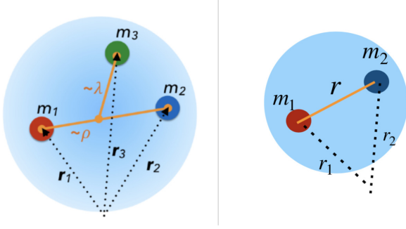
FIG. 1. Illustration of the relative constituent-quark coordinates for mesons and baryons.
