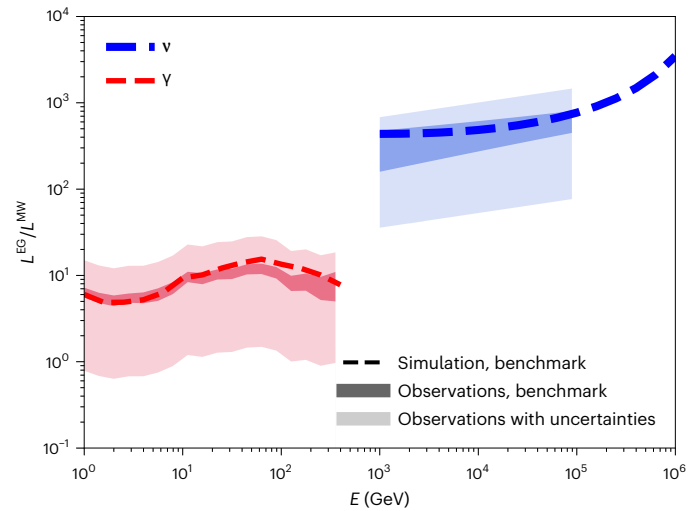
Fig. 2 | Derived ratio of the average luminosity of an external, Milky Way-like Galaxy and the Galactic luminosity in gigaelectronvolt–teraelectronvolt \gamma -rays and teraelectronvolt–petaelectronvolt neutrinos. \gamma -rays are shown in red; neutrinos are shown in blue. The ratio is calculated using equations (1), (2), (4) and (5) with the Fermi-LAT and IceCube measurements of the GDE. The dark-shaded regions adopt the benchmark extragalactic model parameters and assume a uniform emissivity within the Galactic disk. Their widths correspond to the uncertainties in the GDE and EB observations. The dashed curves use not only the benchmark extragalactic model but also a more realistic Galactic model that takes into account the spatial distribution of sources and gas in the Milky Way. The light-shaded region further accounts for the uncertainties in the parameters of the extragalactic model.
