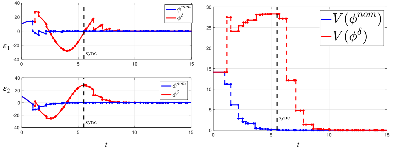
Figure 7 Plot of the error on the state components (left) and of V(x) evaluated along the trajectories of \phi^{nom} and \phi^\delta (right) for the case of initially mismatched clocks \tau_P and \tau_O .
