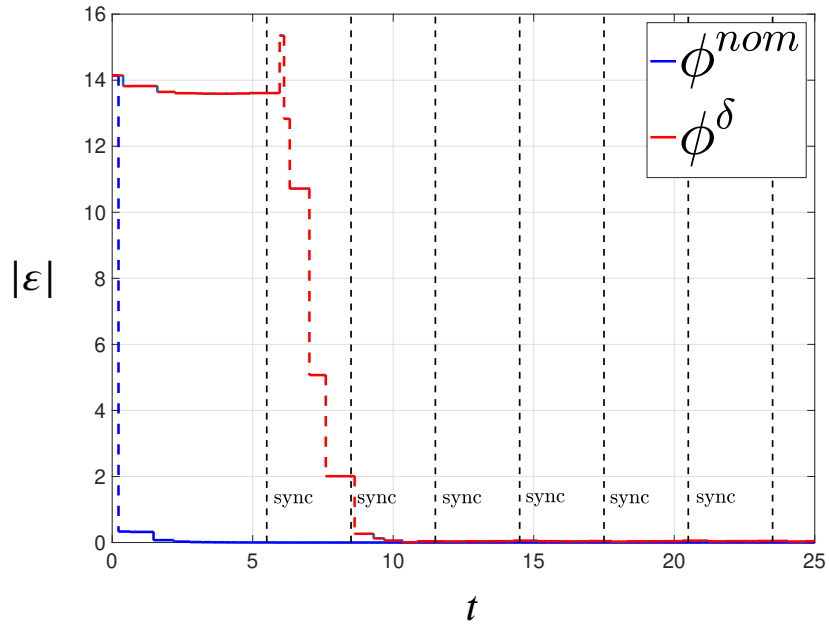
Figure 8 Plot of the error norm for \phi^{\text{nom}} and \phi^\delta with drifting \tau_O clock.
