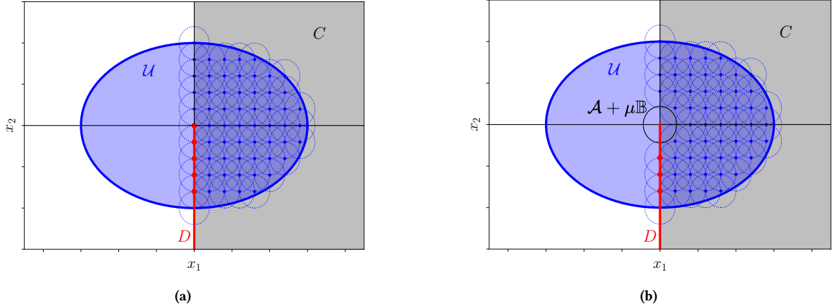
Figure 1: Flow set C , jump set D , sampling set U \subset \mathbb{R}^2 for the oscillator with impacts. In (a), we show the coverings over C \cap U and D \cap U . We enforce conditions at the sampled points (centers of the balls), and under certain assumptions, generalize them to the set U to upper bound the cost associated to solutions to (28). In (b), the \varepsilon -nets cover the sets (C \cap U) \setminus (A + \mu B) and (D \cap U) \setminus (A + \mu B) , respectively, and by extending the conditions enforced at the centers of the balls to the set U , we guarantee practical asymptotic stability of A as in Section 3.2.
