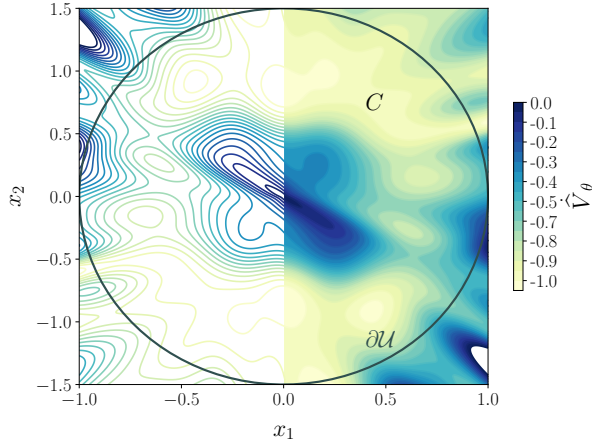
Figure 4: Contour plot of the function x \mapsto \hat{V}_\theta(x) := \langle \nabla \hat{V}_\theta(x), F(x) \rangle . Contours are filled only in the flow set C , which confirms \hat{V}_\theta \leq 0 at C \cap \mathcal{U} .
