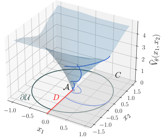
Figure 2: Lyapunov function designed as a neural network trained on the set \mathcal{U} by solving the SP in (11). A hybrid solution to \mathcal{H} from \xi = (1, 0) is shown (in dark blue), illustrating how \hat{V}_\theta decreases along flows and jumps.
