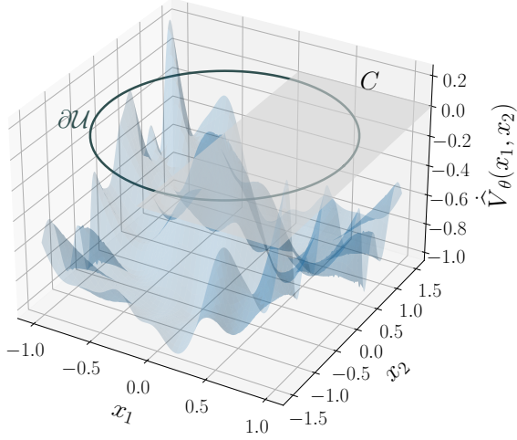
Figure 3: Surface plot of the function x \mapsto \hat{V}_\theta(x) := \langle \nabla \hat{V}_\theta(x), F(x) \rangle . The flow set C and the boundary of the sampling set, namely \partial\mathcal{U} , are displayed. We show that \hat{V}_\theta < 0 at (C \cap \mathcal{U}) \setminus (\mathcal{A} + \mu\mathbb{B}) which is enforced via solving the \text{SP}_\tau in (11) and by Proposition 3.8.
