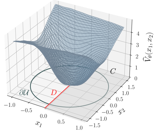
Figure 5: Cost upper bound function designed as a neural network trained on the set \mathcal{U} by solving the SP in (23) for the hybrid oscillator (28). An upper bound on the cost of evolving hybridly from any \xi in (C \cup D) \cap \mathcal{U} is displayed (in blue) with the neural network evaluated at such a point, which does not require computing solutions.
