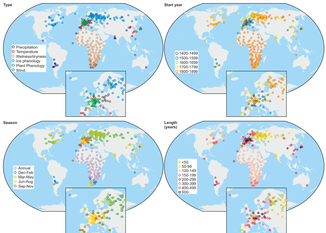
Fig. 6 Map of all documentary data categorized according to (top left) the variable, (top right) the start year, (bottom left) the season covered, and (bottom right) the length.
