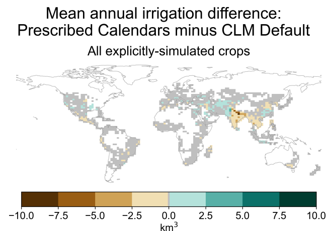
Figure 11. Global distribution of the difference in mean annual irrigation demand, summed across the six crops analyzed here. Gray cells are those outside the top 95 % of cumulative absolute values; white cells had no irrigated crops. See Fig. S26 for positive and negative components in each grid cell and Fig. S27 for maps of individual crops.
